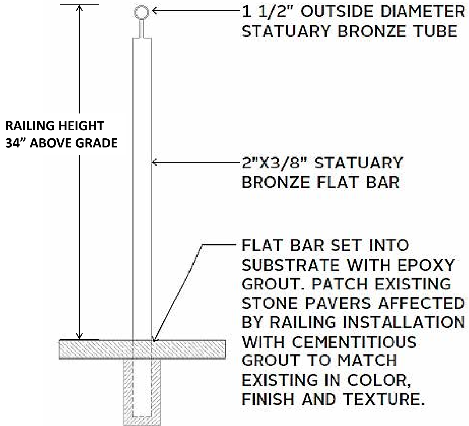
RAILING DETAIL
