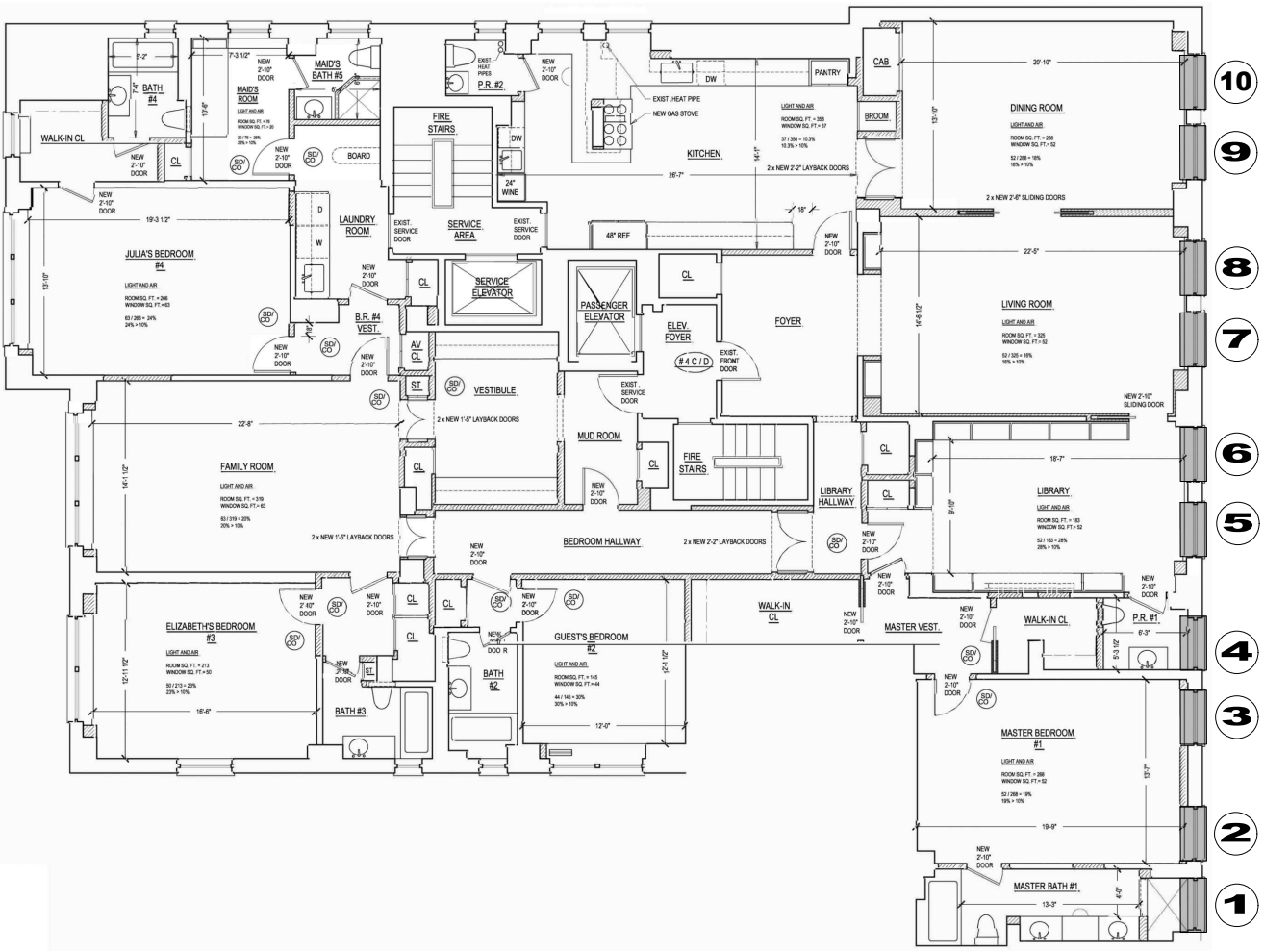
WINDOWS KEY PLAN
