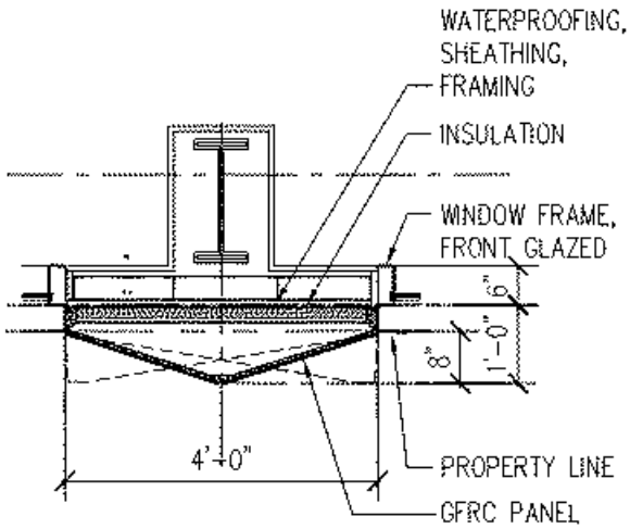
JAMB DETAIL LPC 9/25/2018
