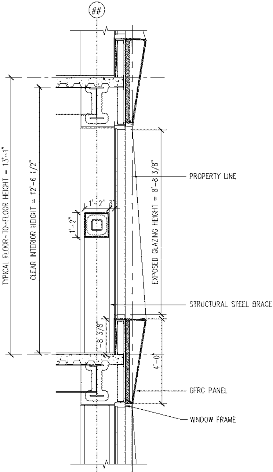
SECTION DETAIL REVISED PROPOSED
