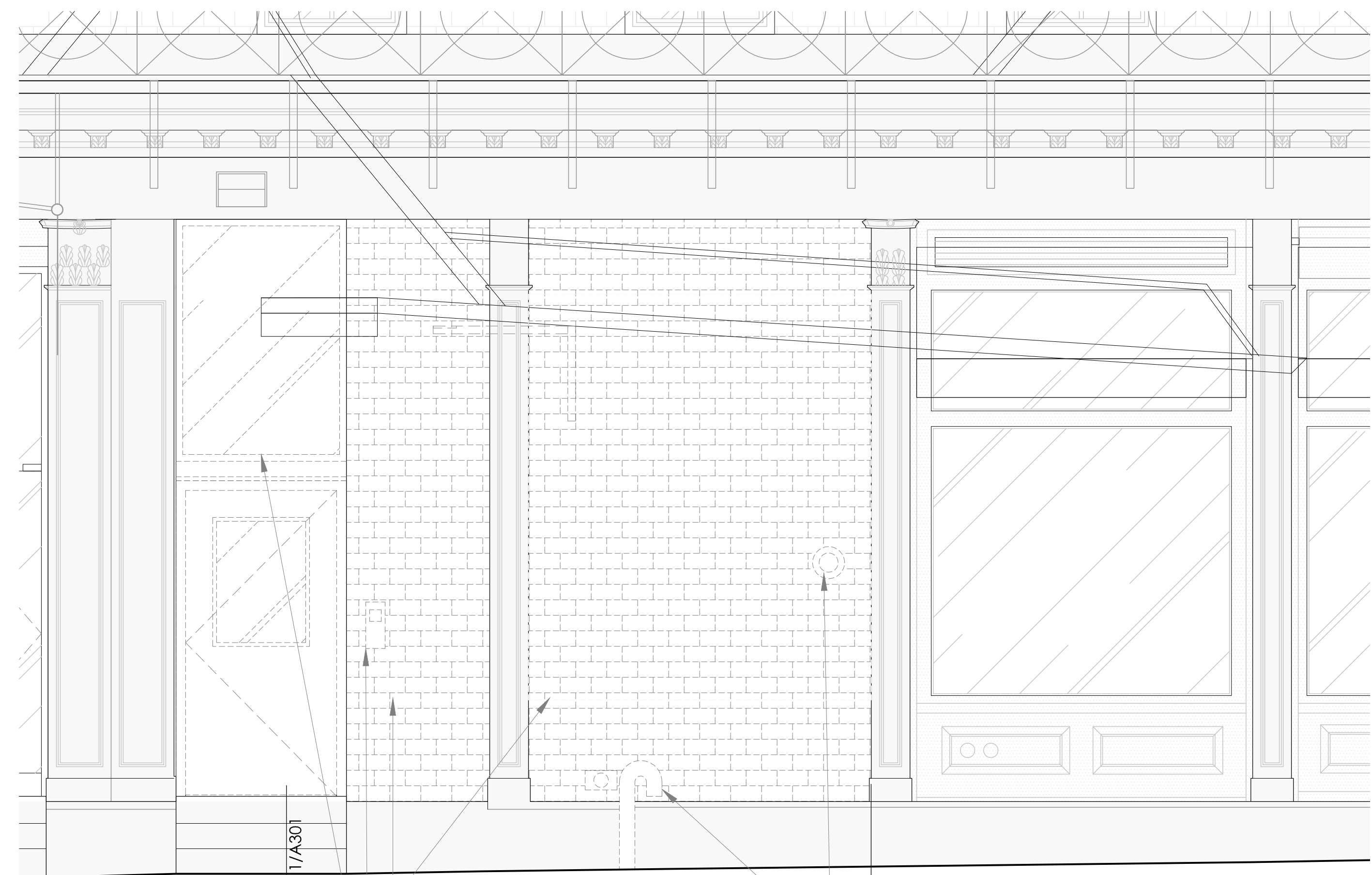
3 ELEVATION - REMOVALS 1/2" = 1'-0"
