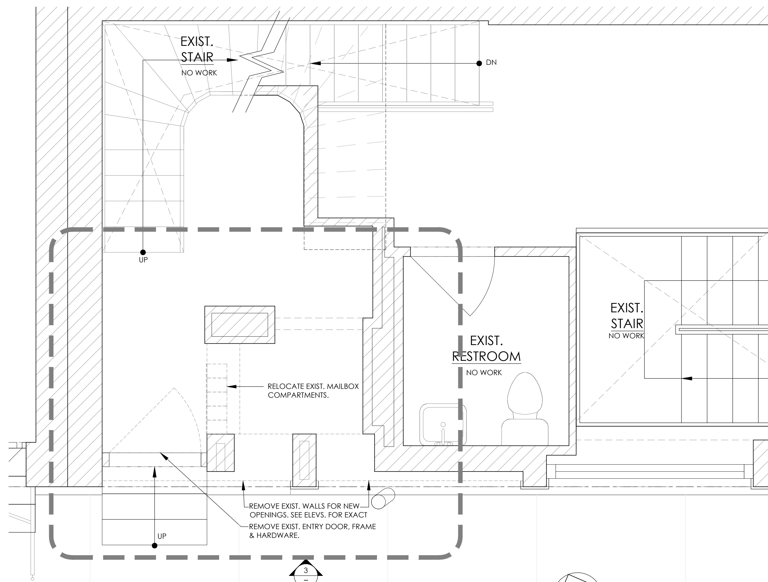
1 REMOVALS PLAN 1/2" = 1'-0"
