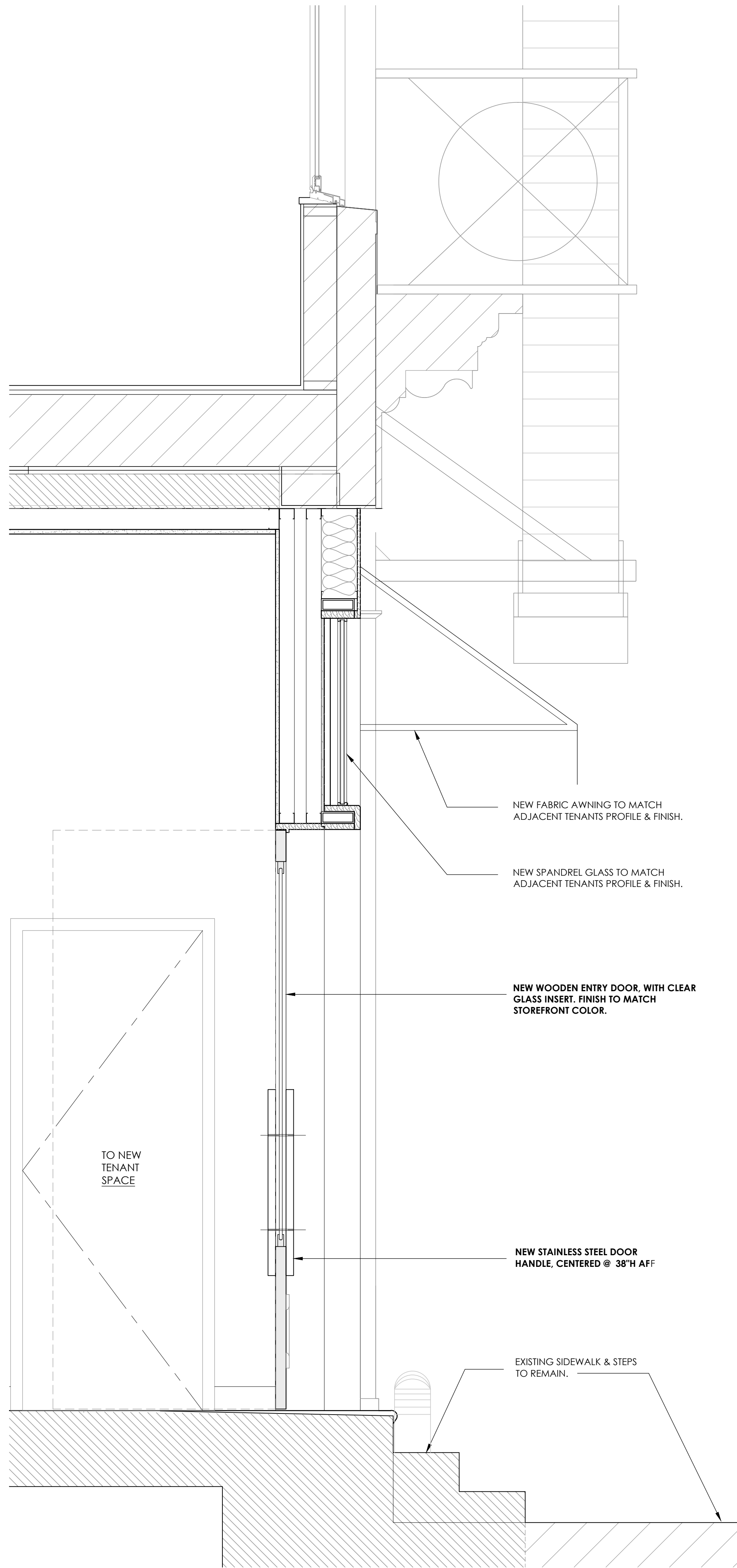
2 SECTION @ ENTRY 1" = 1'-0"
