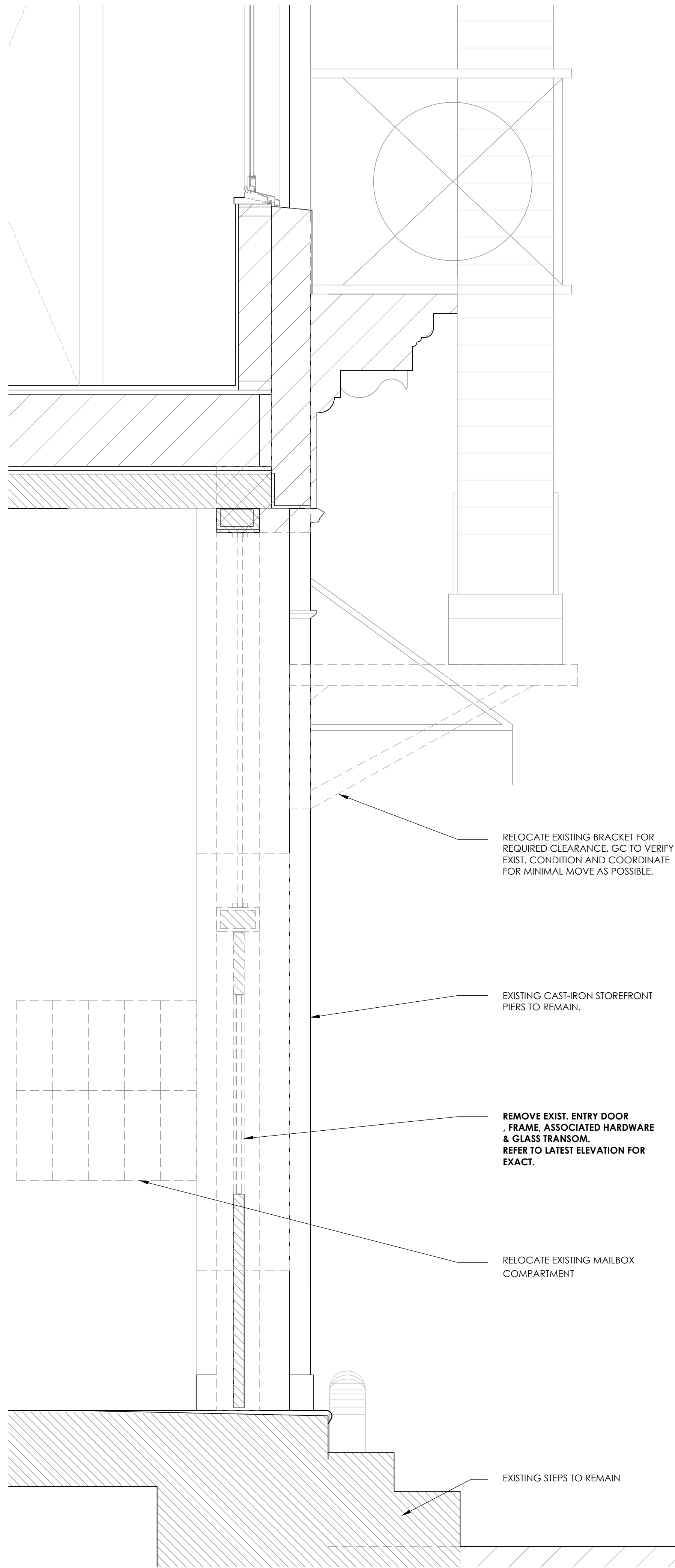
1 SECTION - REMOVALS 1" = 1'-0"
