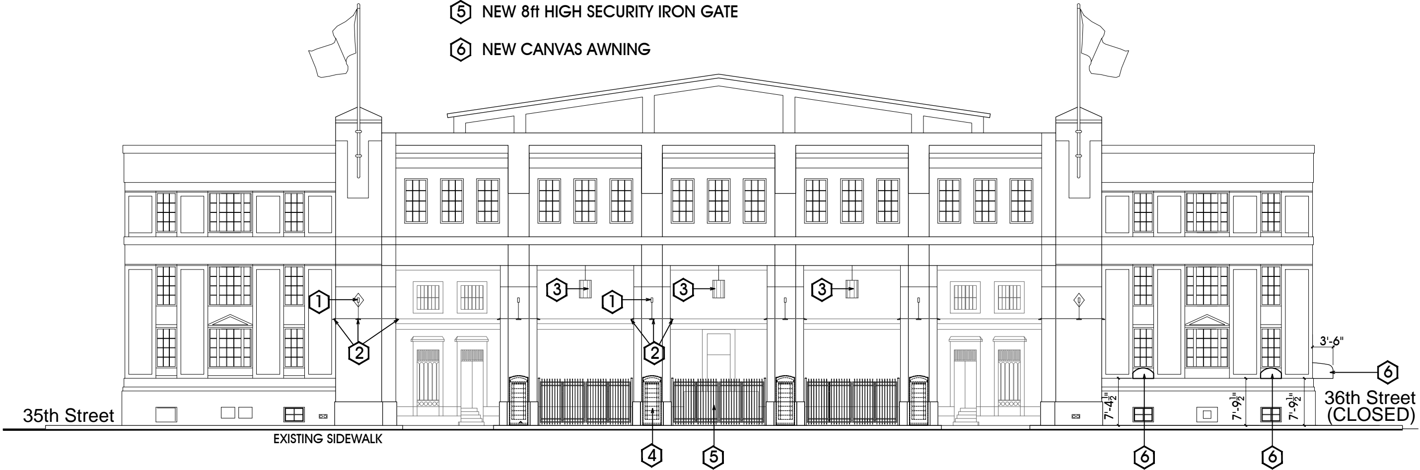
35th Avenue EXTERIOR ELEVATION - PROPOSED FENCE, LIGHTING & AWNINGS
