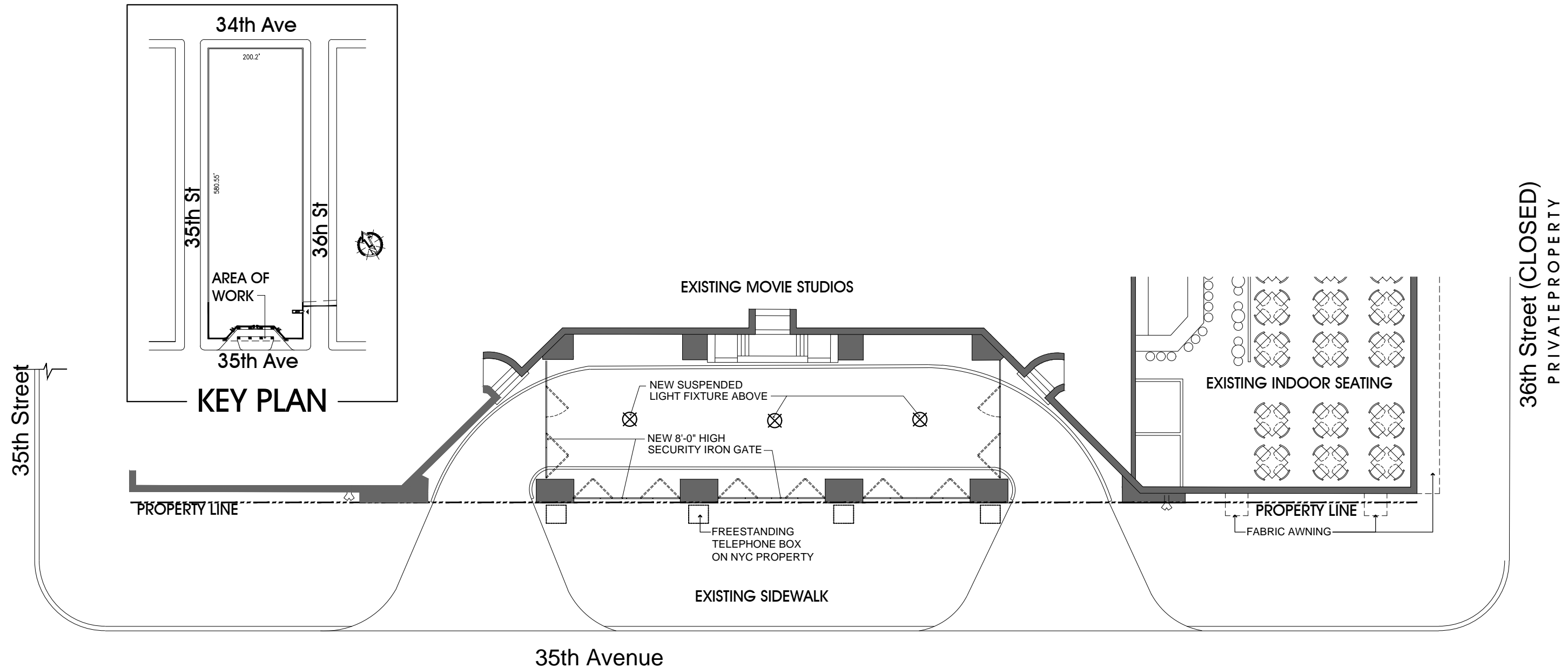
PORTE COCHERE PROPOSED FENCE, LIGHTING AND AWNINGS PLAN VIEW
