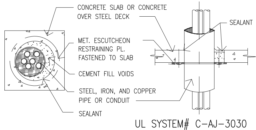
TYPICAL FIRESTOPPING DETAILS
