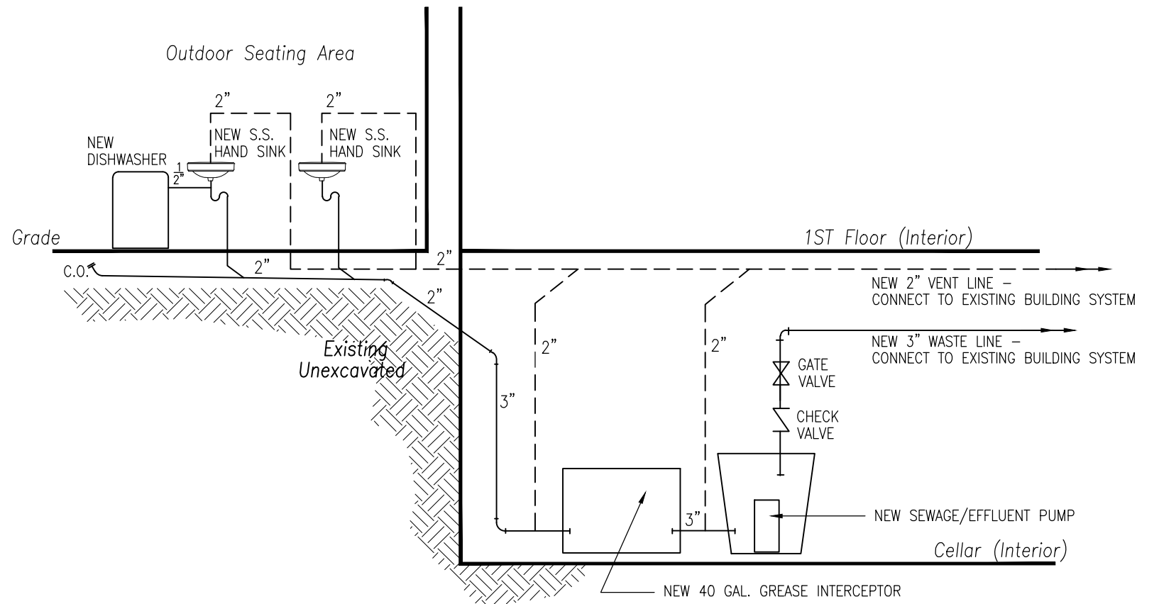
SANITARY RISER DIAGRAM
