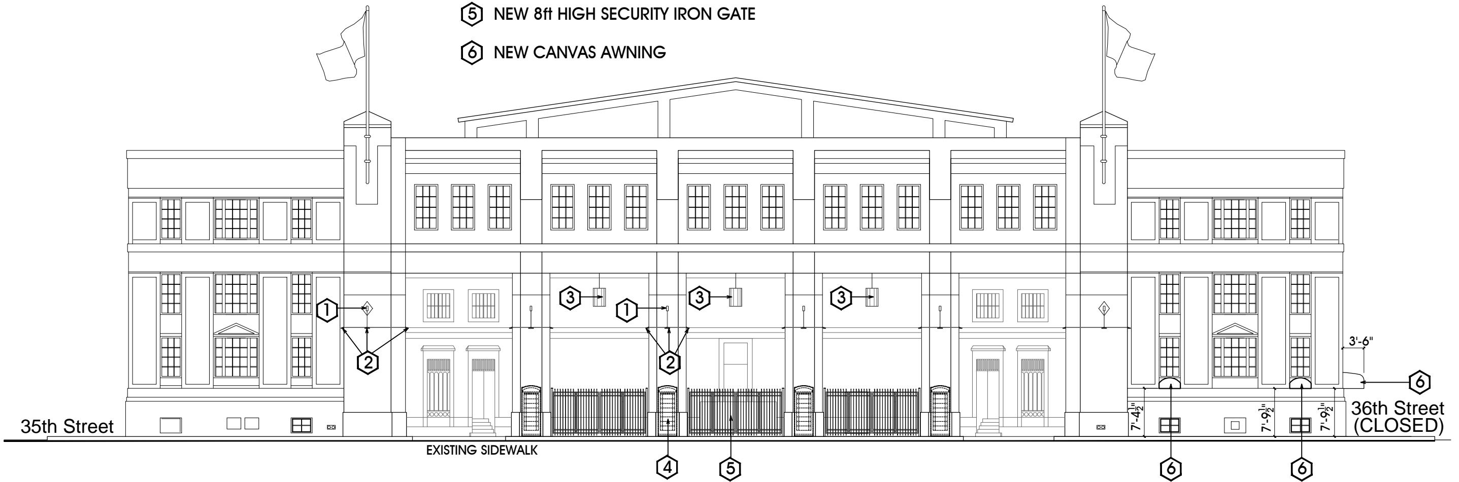
35th Avenue EXTERIOR ELEVATION - GEORGE'S OUTDOOR CAFE
