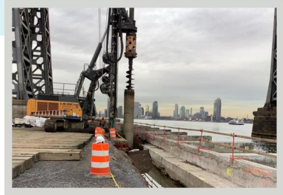
Combi-wall installation underneath Williamsburg Bridge, January 2023
