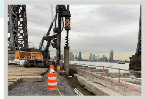
Combi-wall installation underneath Williamsburg Bridge, January 2023
