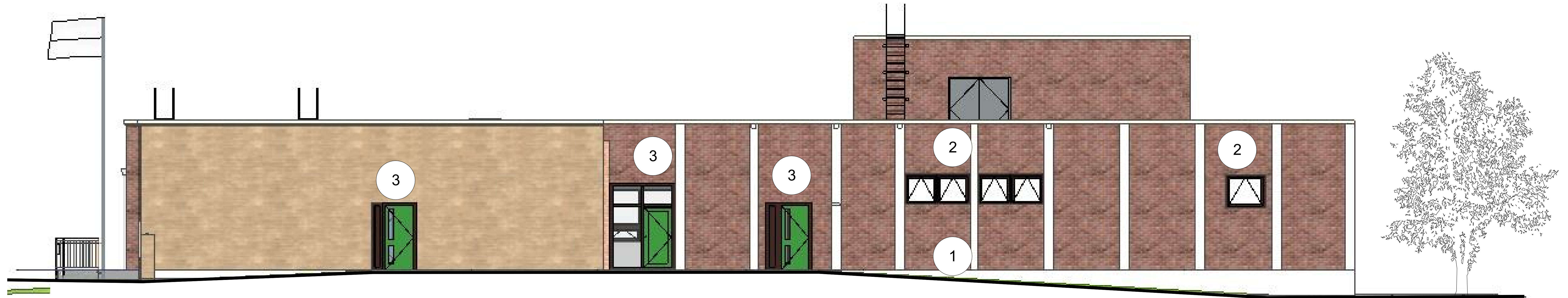
1 PROPOSED NORTH ELEVATION SCALE: 3/16" = 1'-0"
