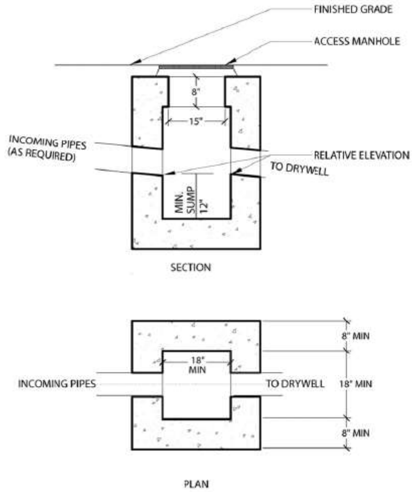
FIGURE 1114.4(1): GRIT CHAMBER
