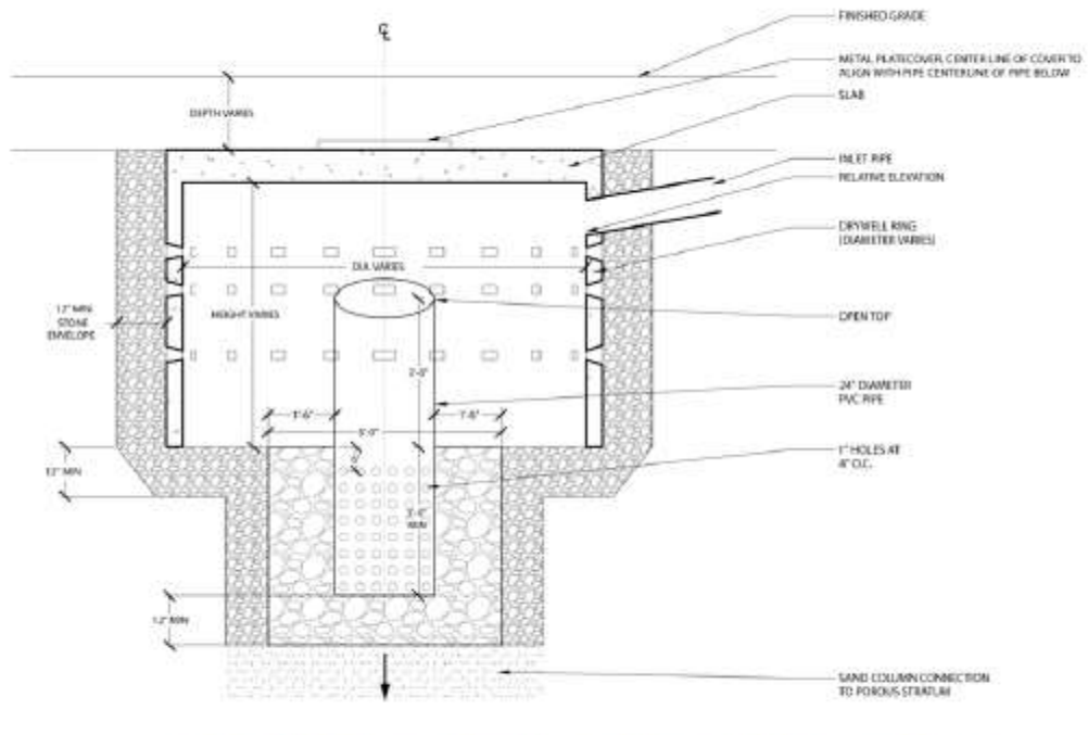
FIGURE 1114.4(2) DETAIL OF DRYWELL WITH SAND COLUMN
