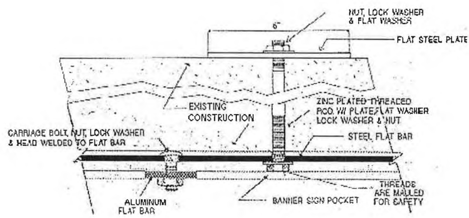
DETAIL A-2 THRU BOLT INSTALLATION PLAN ( AT EACH END )
