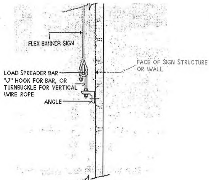
SECTION C SECUREMENT TO RESTRAINING ANGLES
