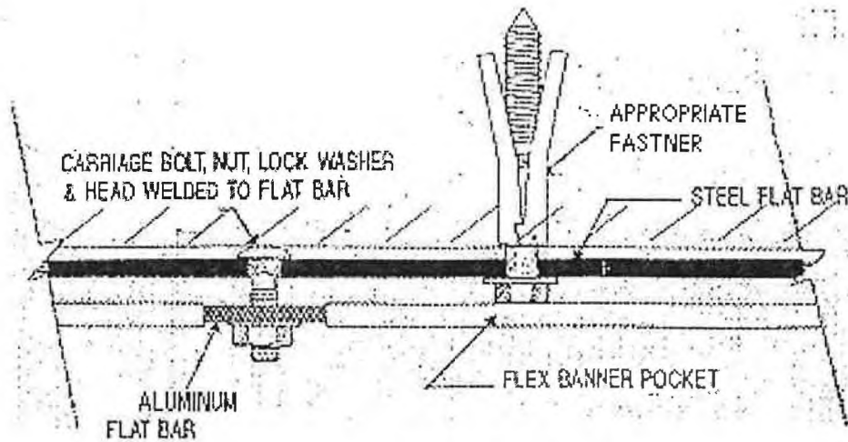
DETAIL A-1 WALL ANCHOR INSTALLATION PLAN
