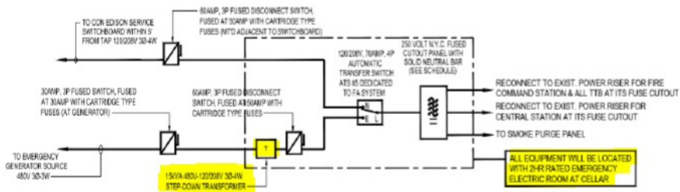
DETAIL OF FIRE ALARM SYSTEM POWER SUPPLY FROM 120/208V NORMAL AND 480V EMERGENCY SERVICES
