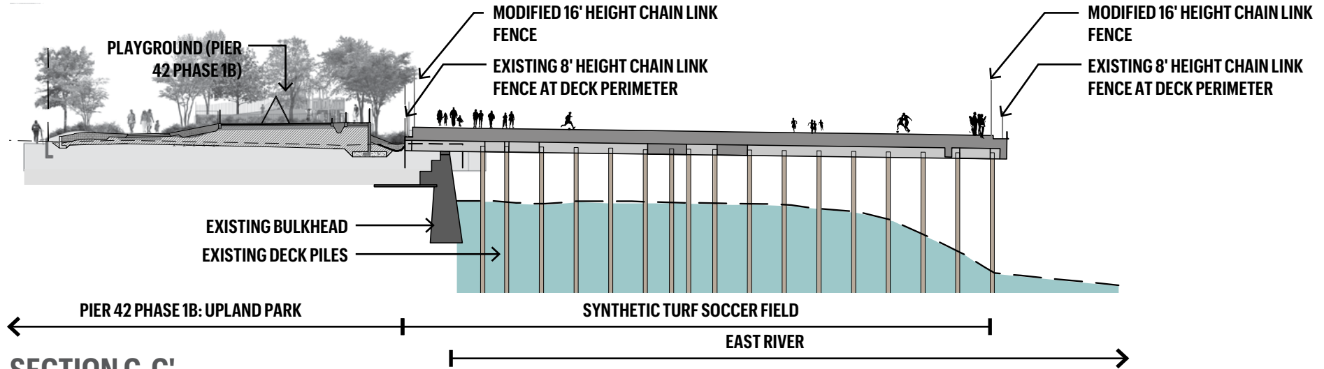
SECTION C-C'
