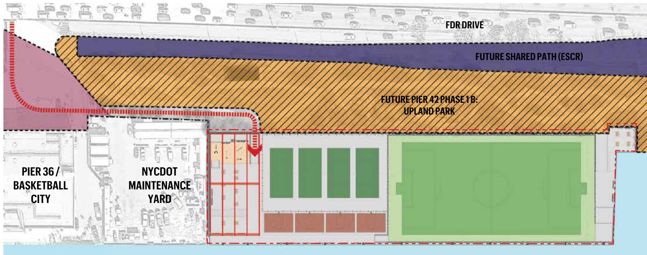
DECK ACCESS DURING PHASE 1B CONSTRUCTION
