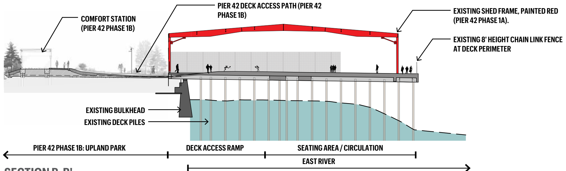
SECTION B-B'
