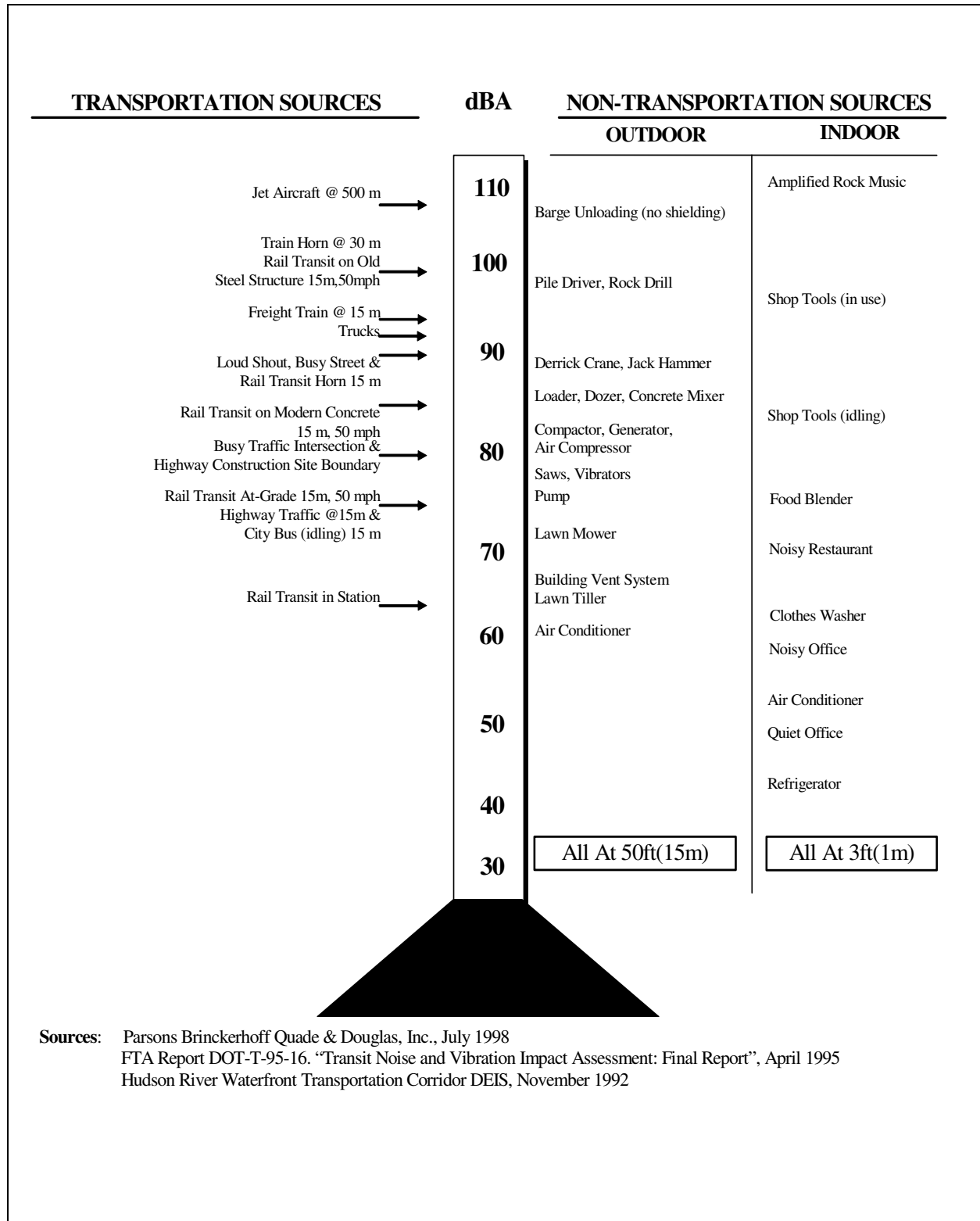
Figure 18-1 Common Indoor and Outdoor Noise Levels
