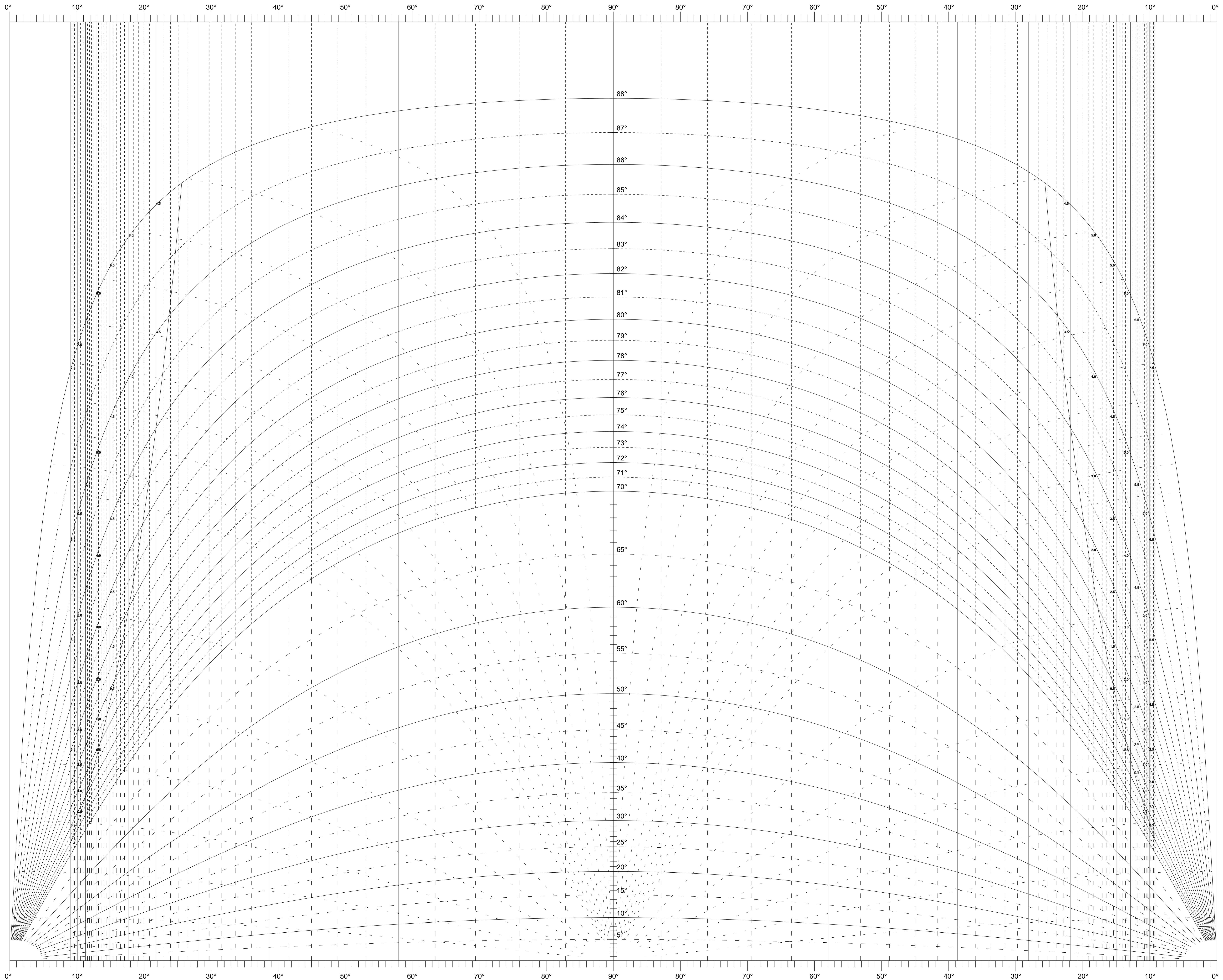
DAYLIGHT EVALUATION DIAGRAM - 80 FOOT STREET
