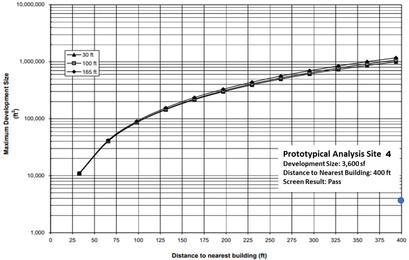
FIG App 17-5 SO 2 BOILER SCREEN RESIDENTIAL DEVELOPMENT - FUEL OIL #2
