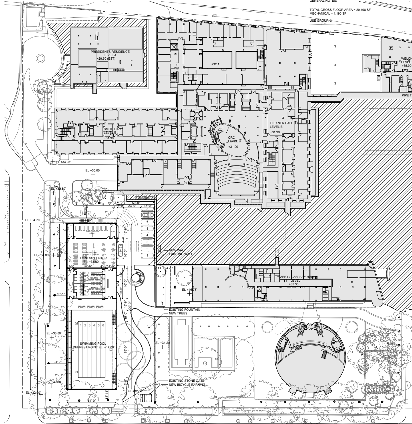
LEVEL 1 PLAN
