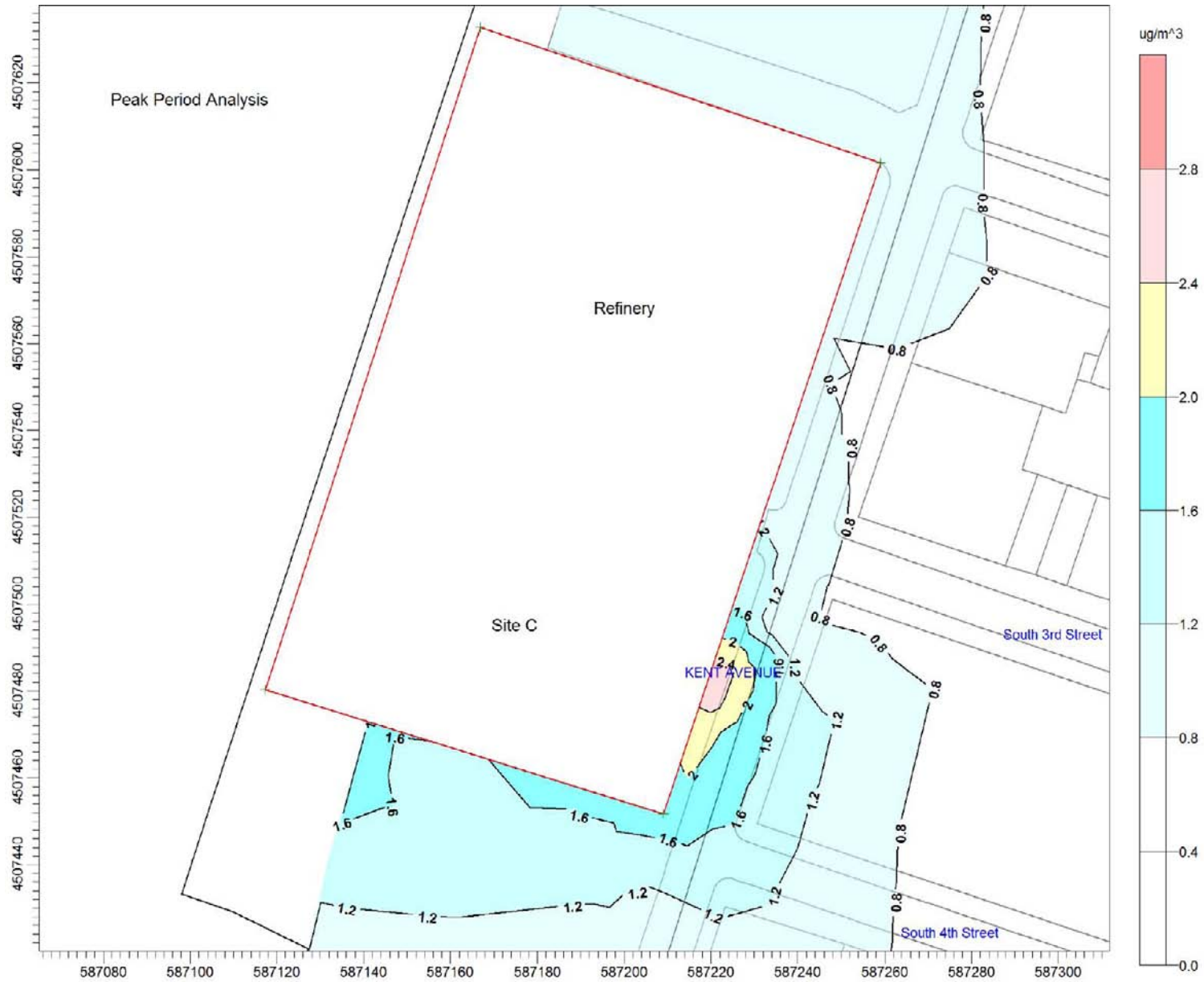
Maximum Predicted 24-Hour Average Increase in PM 2.5 Concentration Peak Period Analysis Figure G-10
