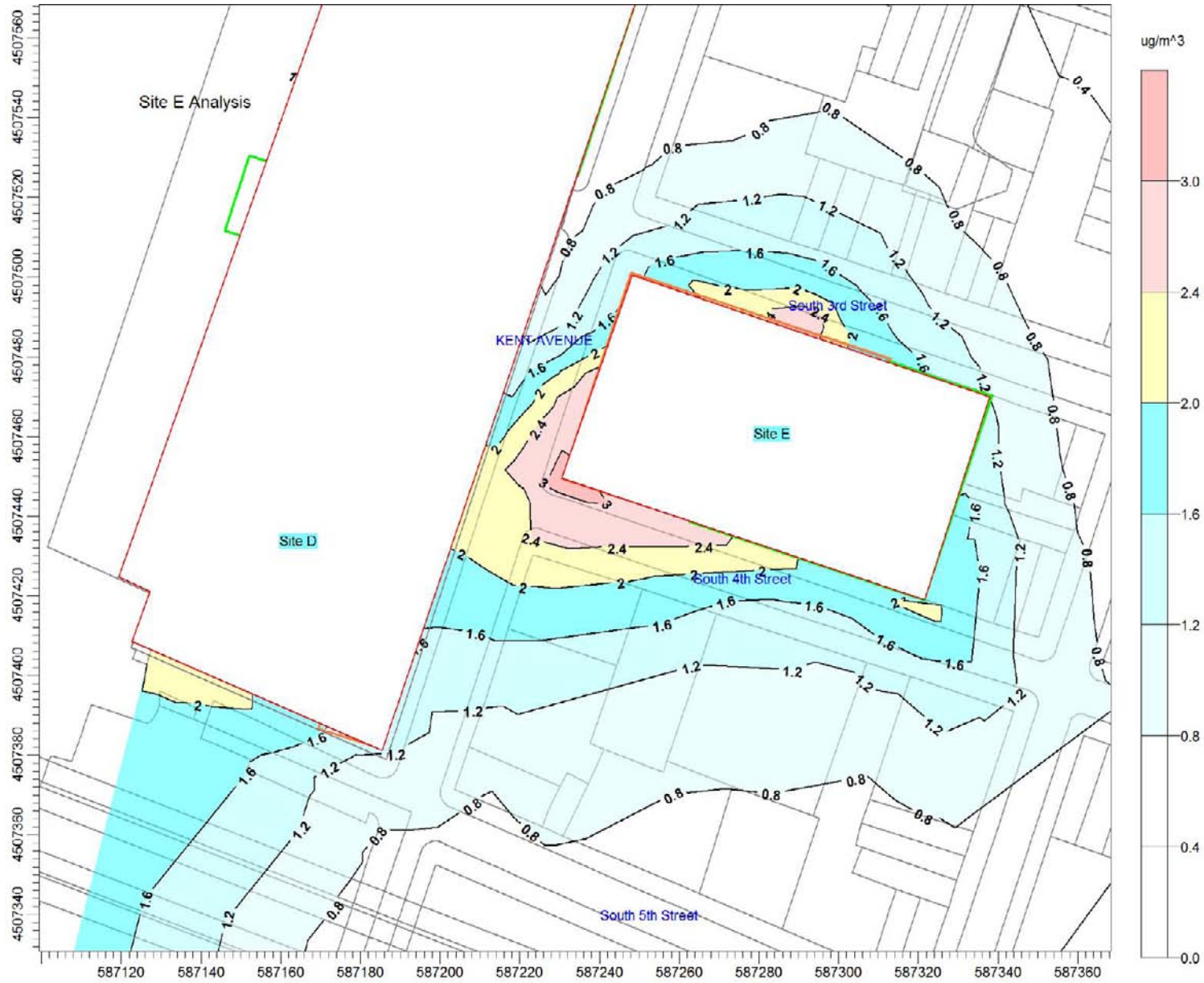
Maximum Predicted 24-Hour Average Increase in PM 2.5 Concentration Site E Analysis Figure G-12
