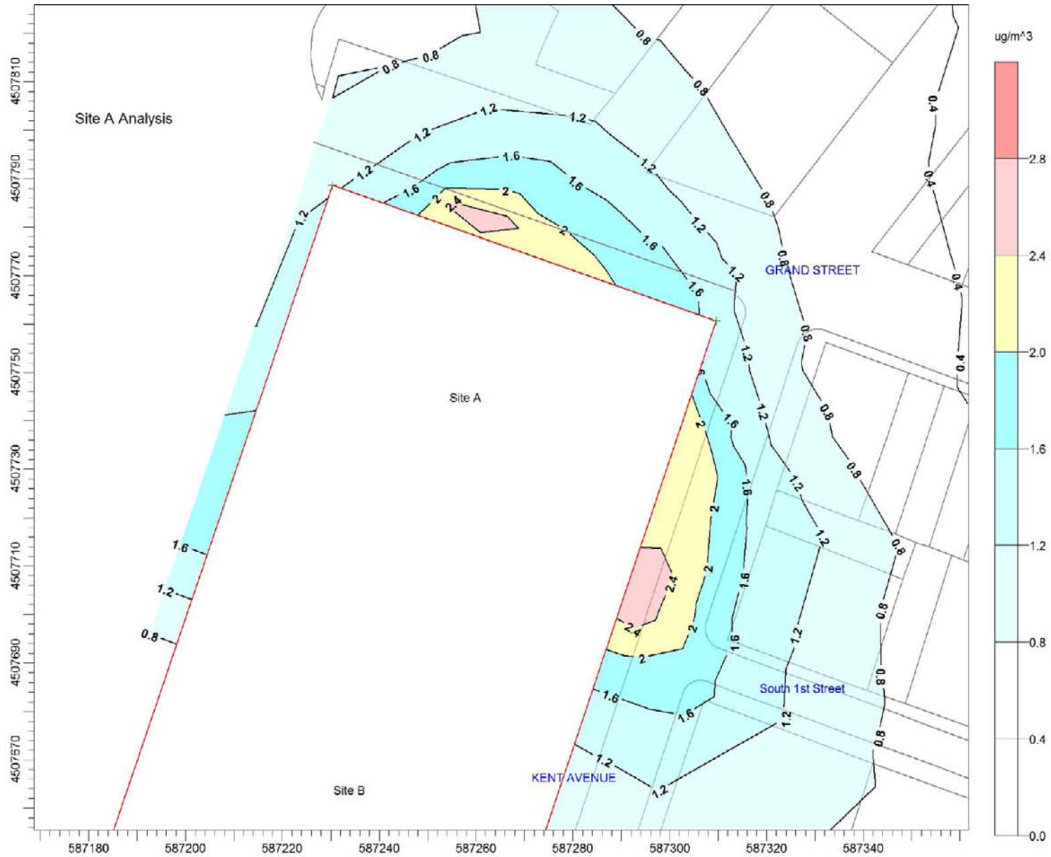
Maximum Predicted 24-Hour Average Increase in PM 2.5 Concentration Site A Analysis Figure G-11
