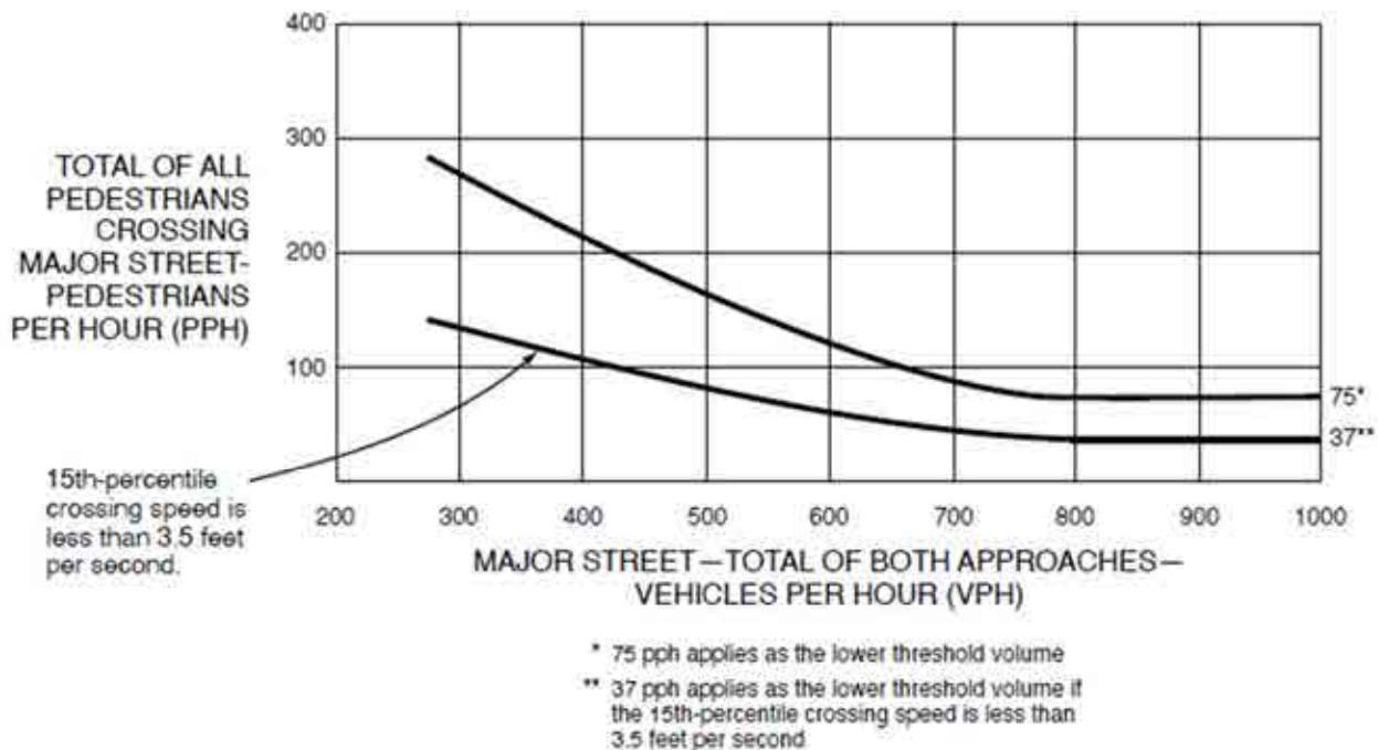
Figure 4C-7. Warrant 4, Pedestrian Four-Hour Volume (70% Factor) (COMMUNITY LESS THAN 10,000 POPULATION OR ABOVE 40 MPH ON MAJOR STREET)
