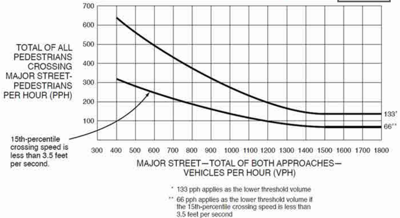
Figure 4C-6. Warrant 4, Pedestrian Peak Hour
