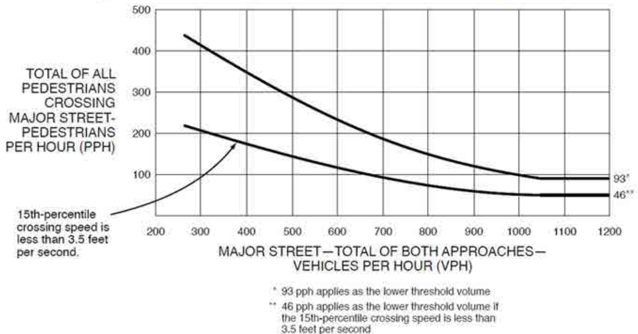
Figure 4C-8. Warrant 4, Pedestrian Peak Hour (70% Factor)
