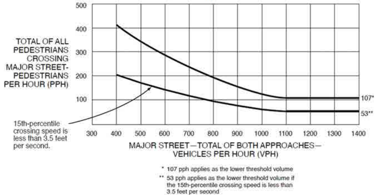
Figure 4C-5. Warrant 4, Pedestrian Four-Hour Volume
