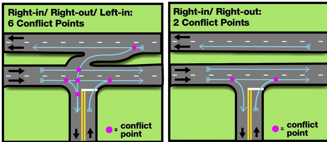
Figure 16-4 Vehicle to Vehicle Conflict Points at a Driveway with Non-Traversable Median
