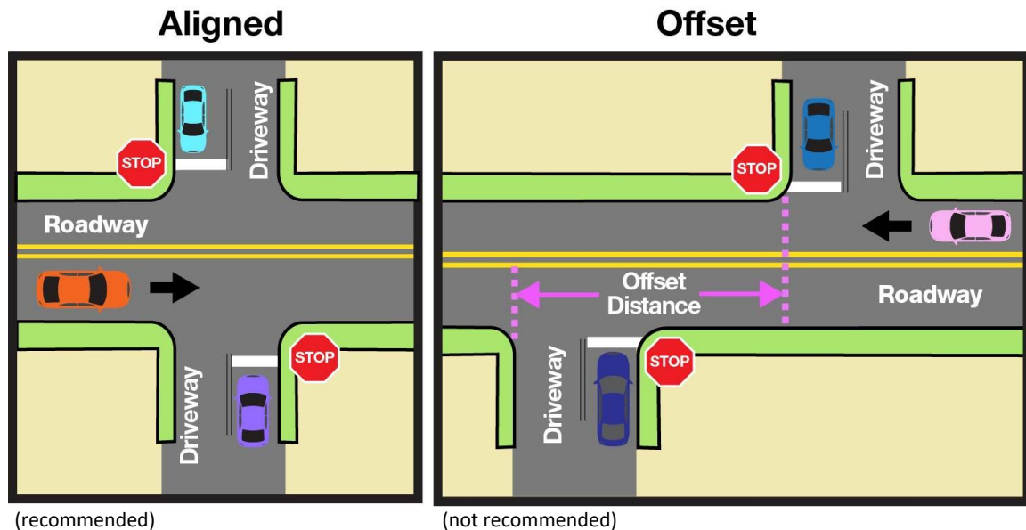
Figure 16-7 Aligned versus Offset Driveway Spacing
