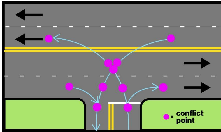
Figure 16-3 Vehicle to Vehicle Conflict Points (11) at a Full-Access Driveway (No Median)
