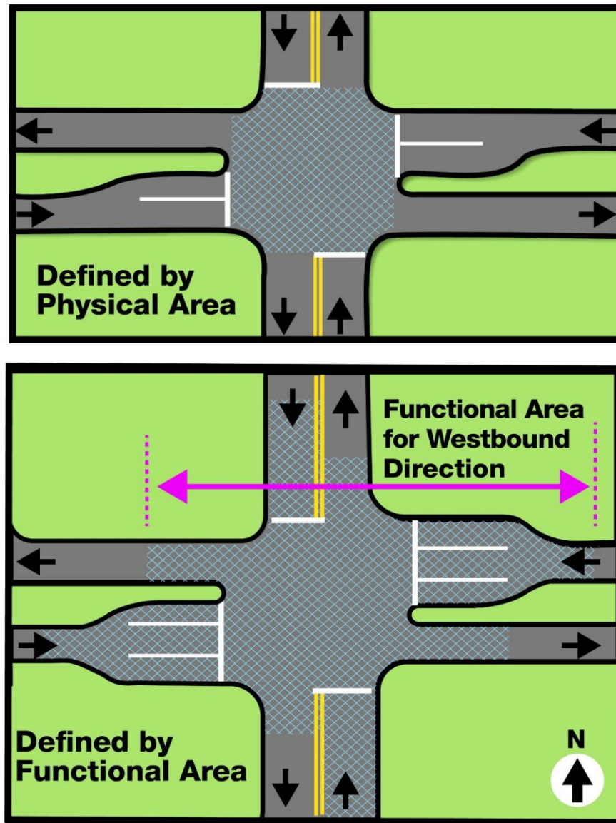
Figure 16-2 Intersection Functional Area versus Intersection Physical Area
