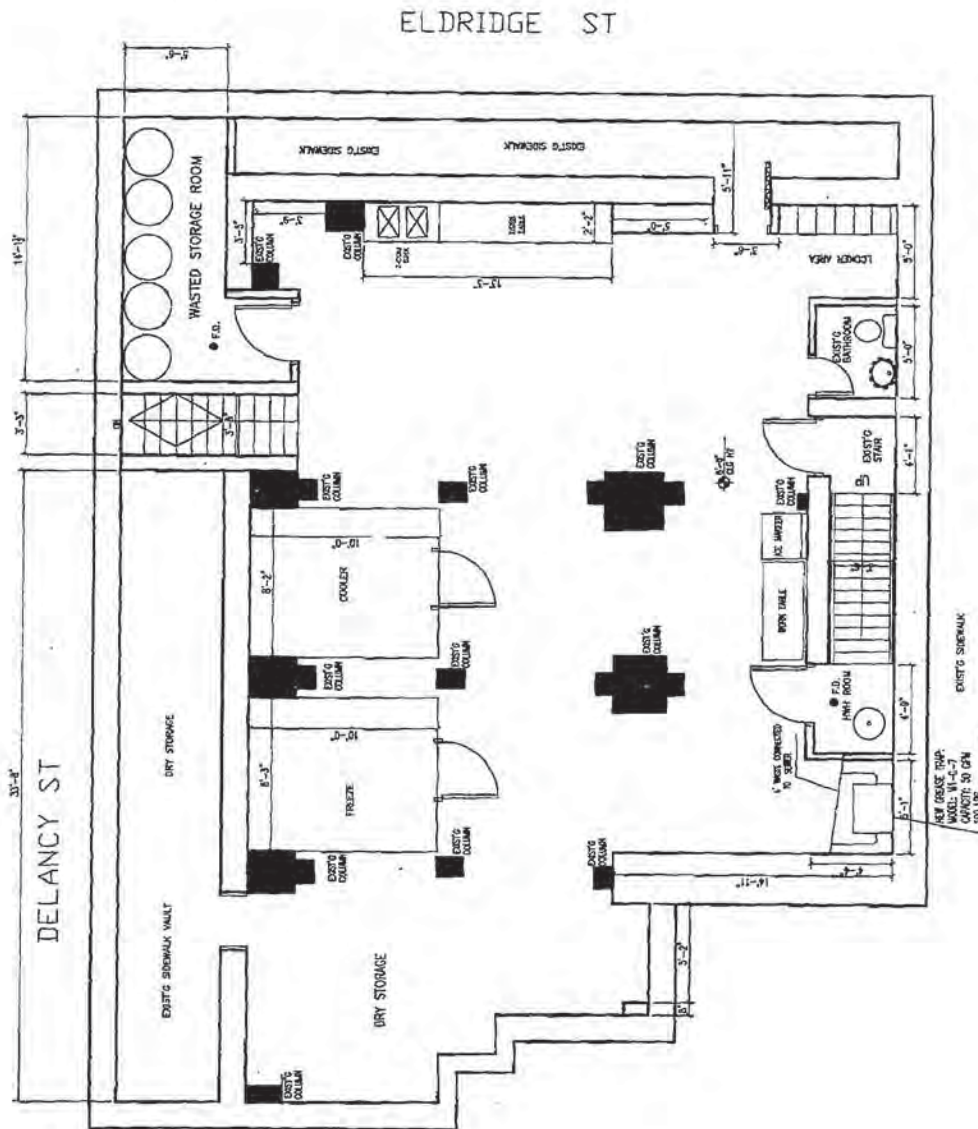
PROPOSED BASEMENT FLOOR PLAN 1/4"=1'
