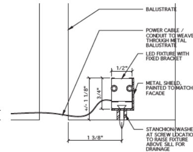
LIGHTING FIXTURE DETAIL - EX03
