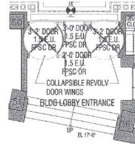
current vestibule door and revolving door configuration
