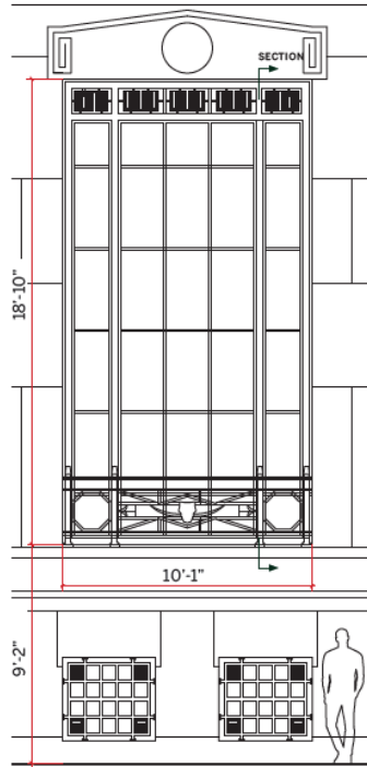
WINDOW ELEVATION
