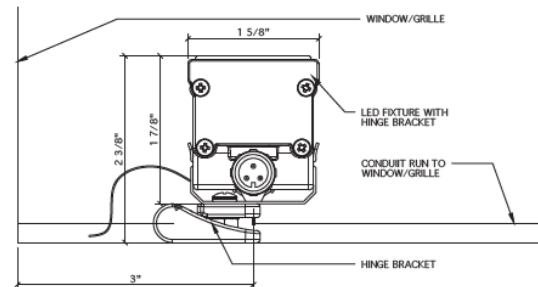
LIGHTING FIXTURE DETAIL - EX02
