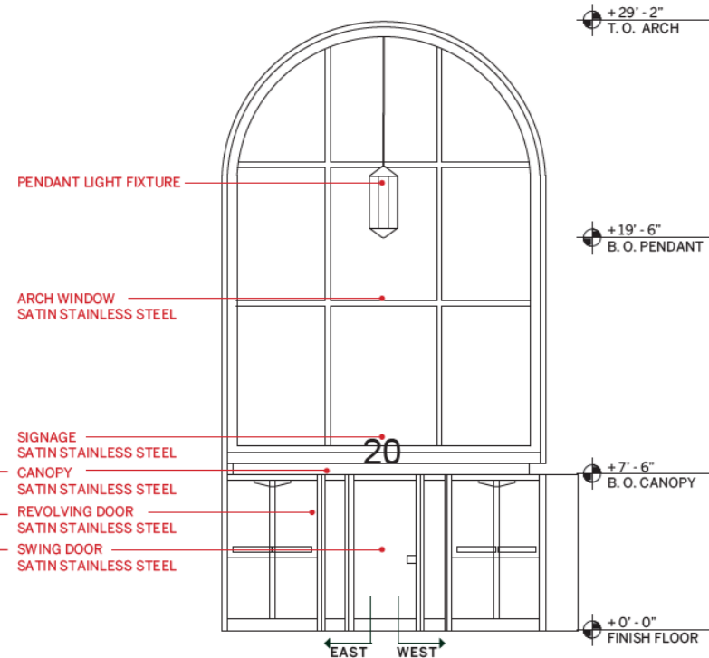
EXG EXCHANGE PLACE ENTRANCE ELEVATION
