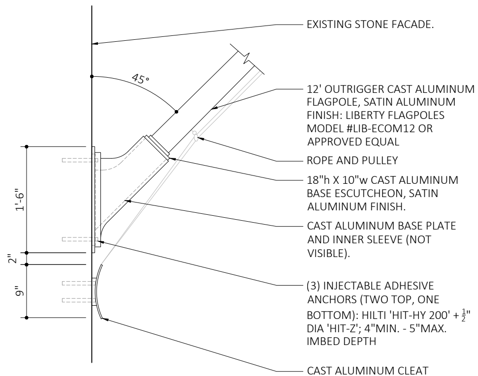
2 BASE DETAIL FOR PROPOSED FLAGPOLE 3/4"=1'-0"
