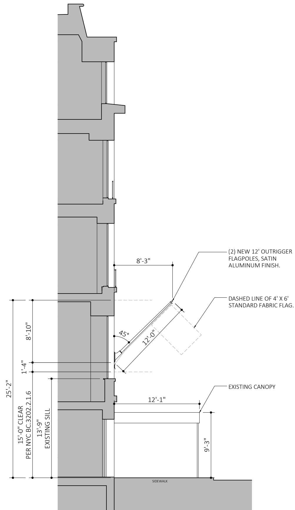
1 PRIMARY FACADE SECTION - PROPOSED 1/8"=1'-0"
