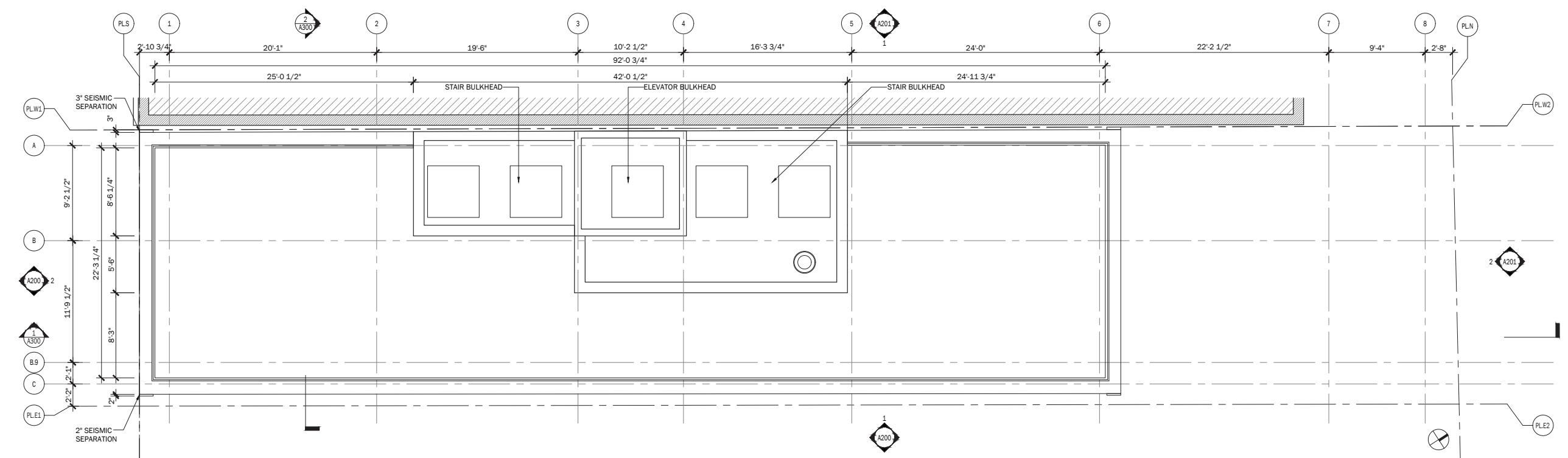
2 BULKHEAD PLAN 3/16"=1'-0"
