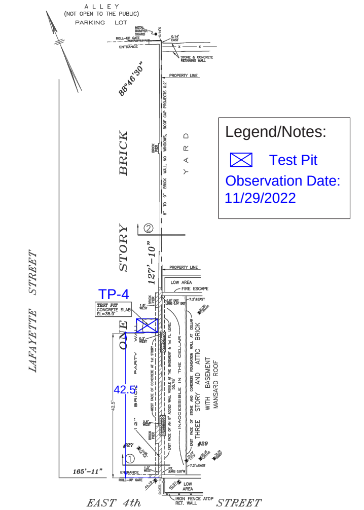
TEST BORINGS LOCATION PLAN
