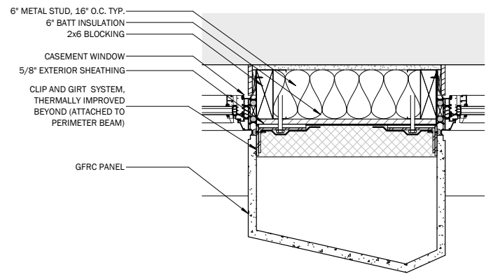
2 PLAN SECTION DETAIL - TYP. GFRP PANEL TO GLASS 1 1/2" = 1'-0"
