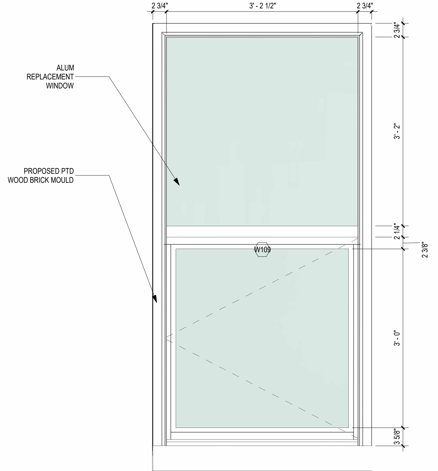
3 PROPOSED DOUBLE-HUNG WINDOW ELEVATION DETAIL 1" = 1'-0"
