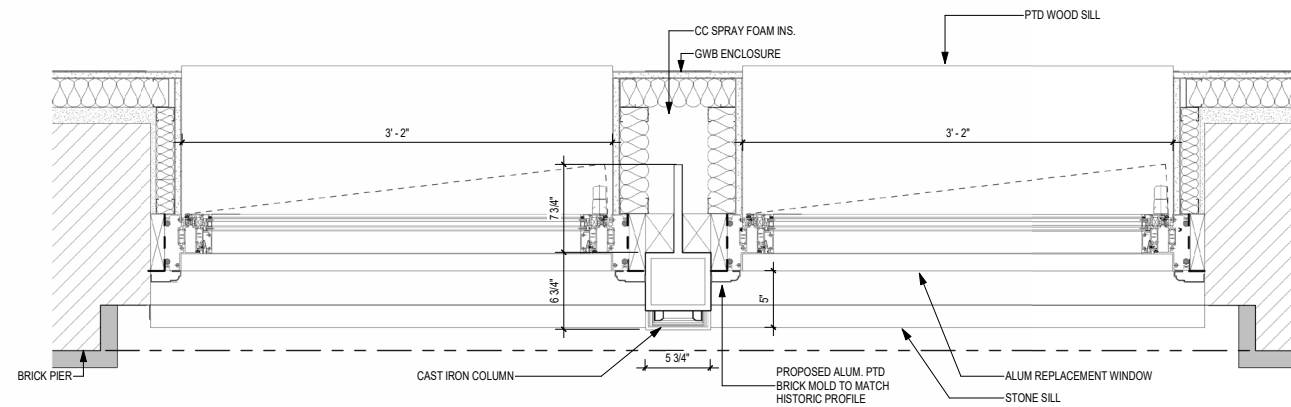
⑦ TYPICAL WINDOW PLAN PROPOSAL 1 1/2" = 1'-0"
