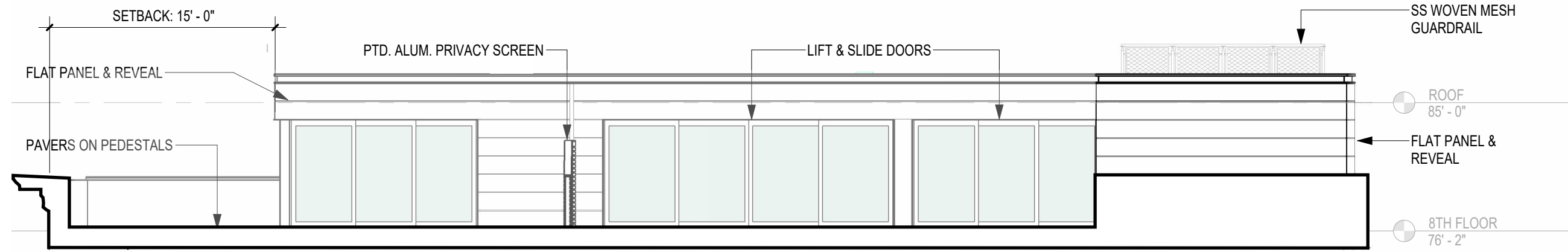
① PH ADDITION - WEST ELEVATION - MOTT ST 1/8" = 1'-0"
