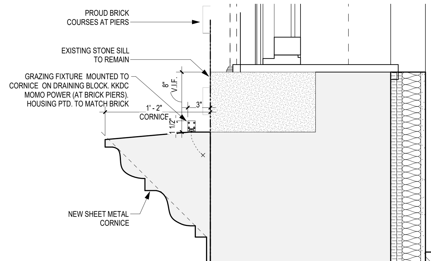
GRAZING LIGHT FIXTURE AT BRICK PIERS
