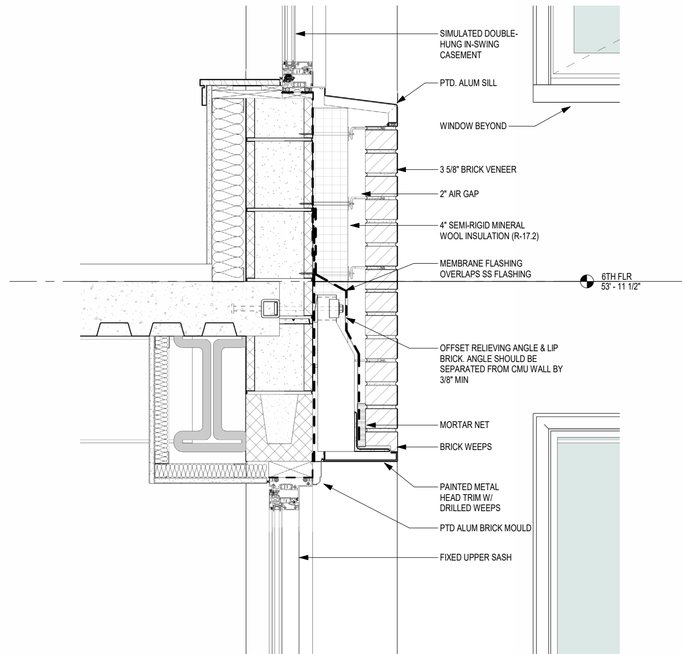
① EAST COURTYARD DETAIL AT WINDOW 1 1/2" = 1'-0"
