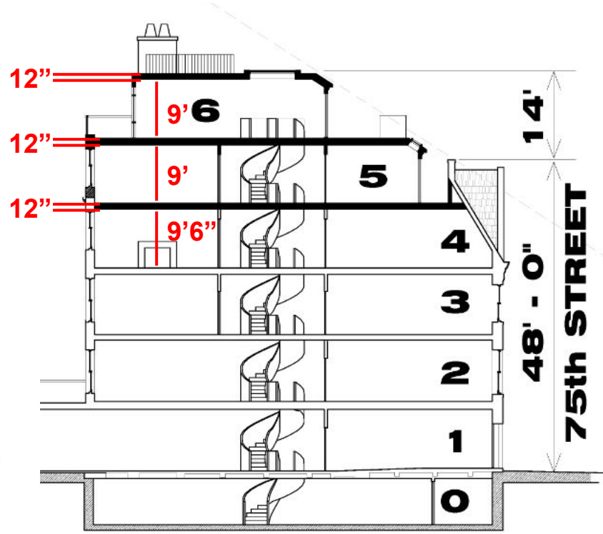
PROPOSED SECTION
