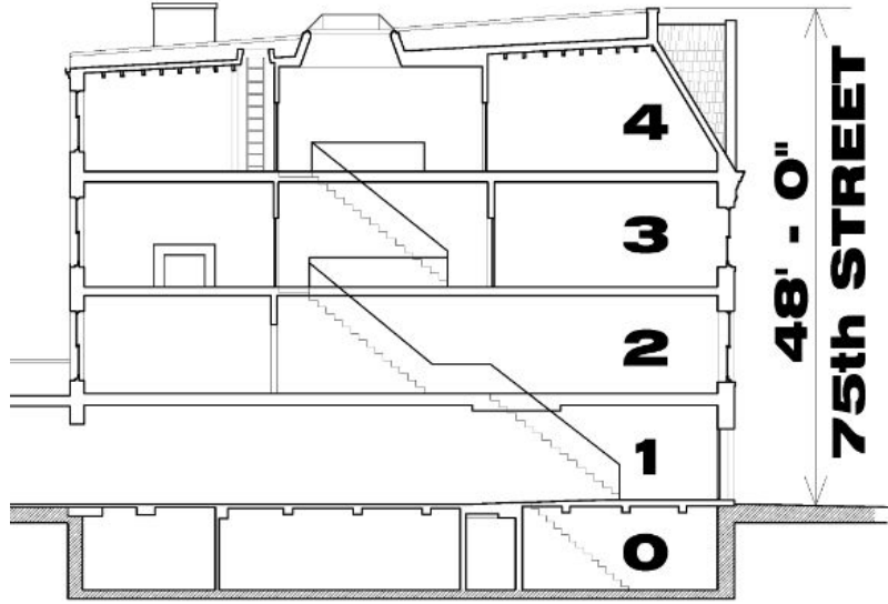
EXISTING SECTION
