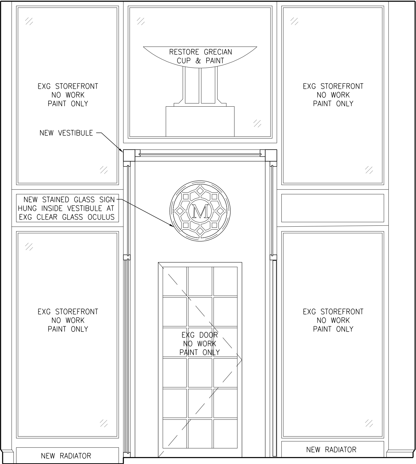
PROPOSED INTERIOR VESTIBULE ELEVATION
