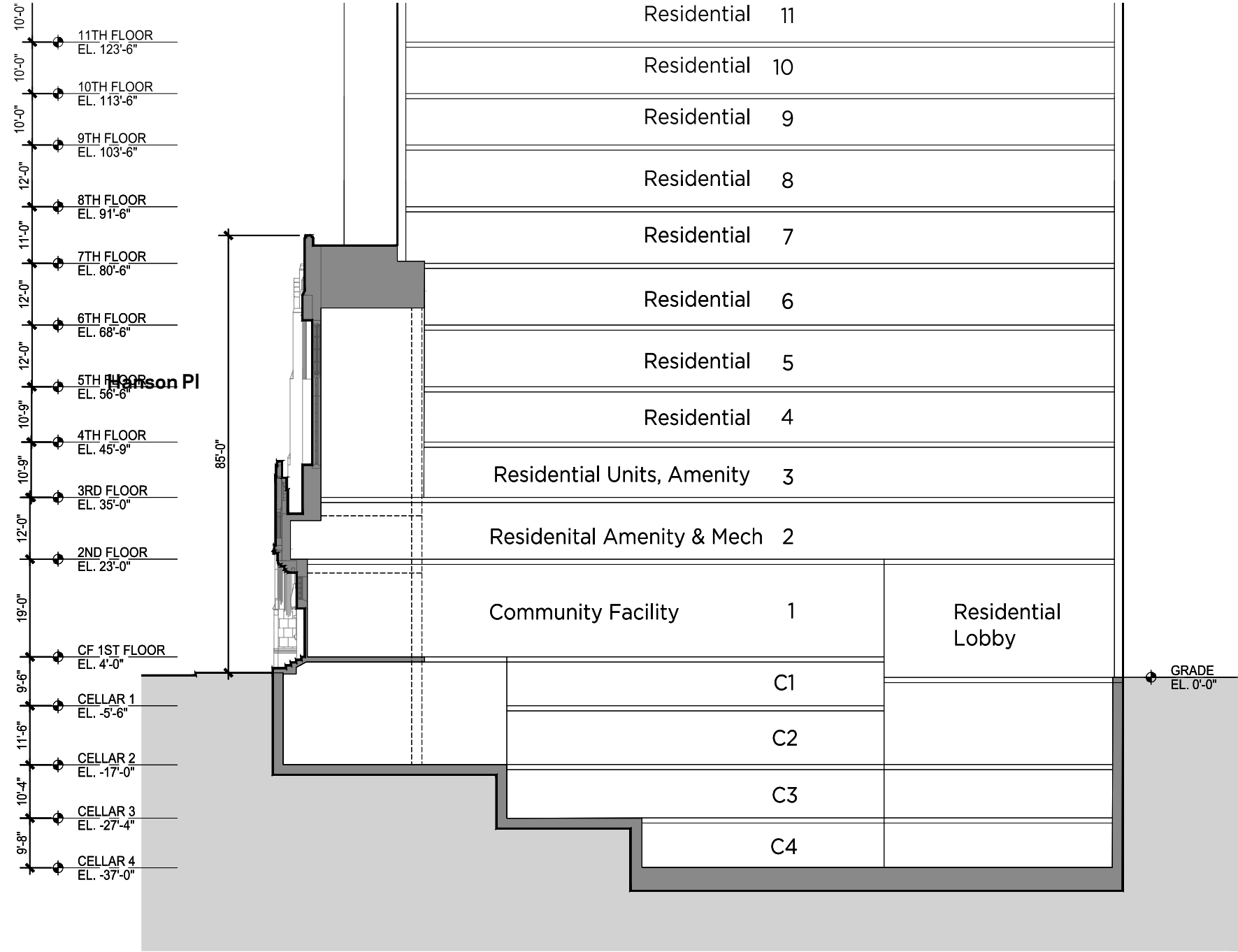
North-South Section
