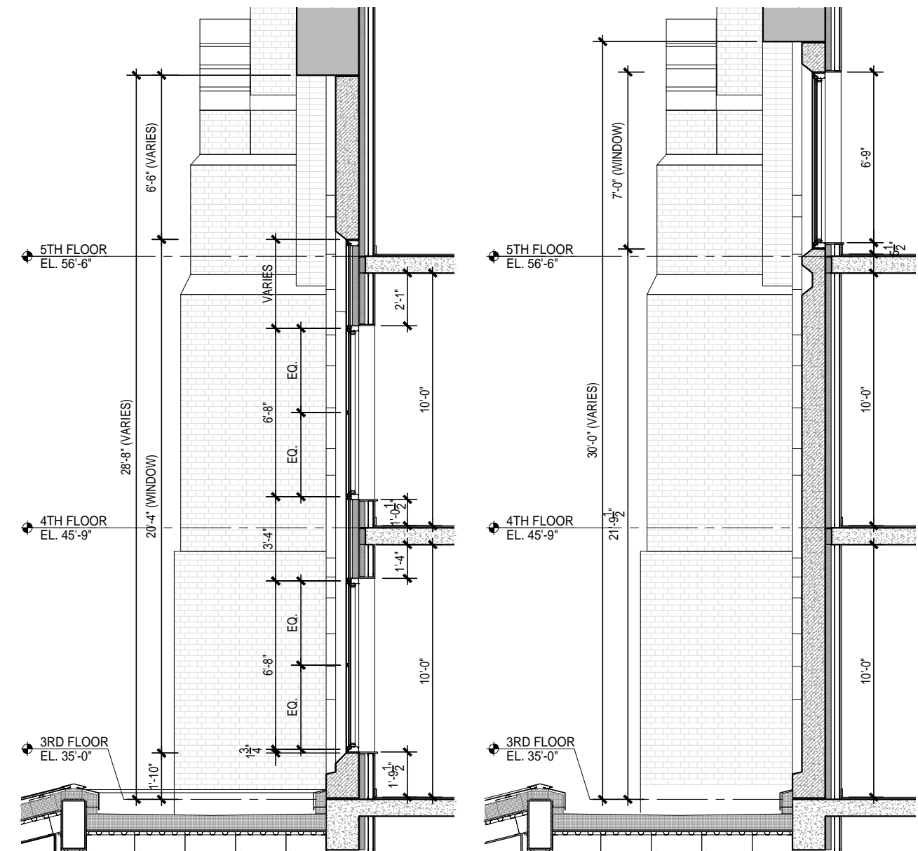
3 SECTION 3/16" = 1'-0"
