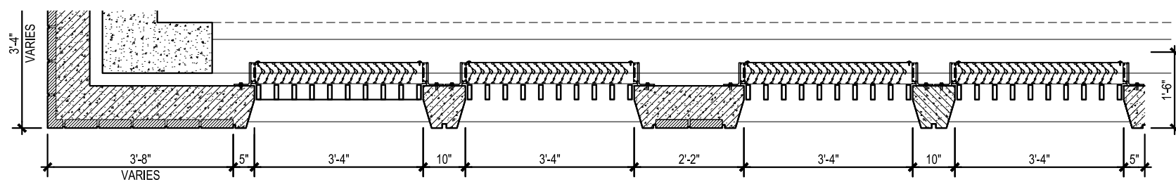
1 ELEVATION 3/8" = 1'-0"
