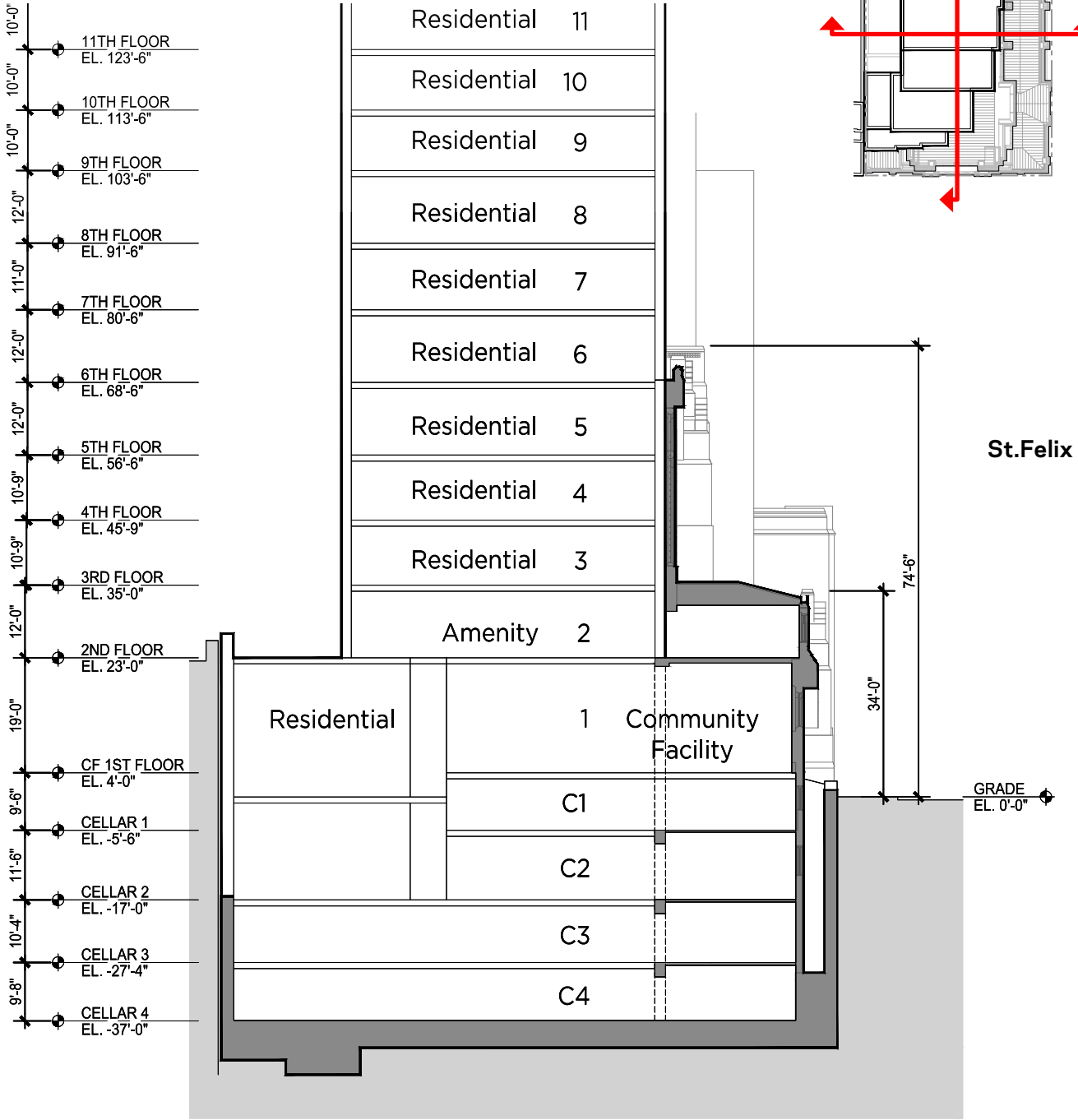
East-West Section
