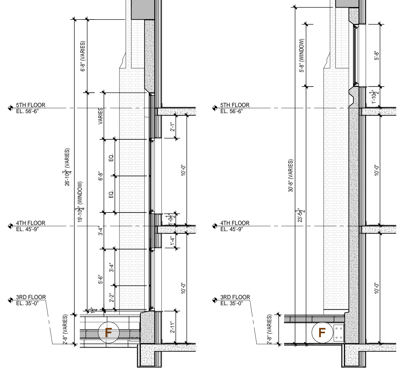
3 SECTION 3/16" = 1'-0"
