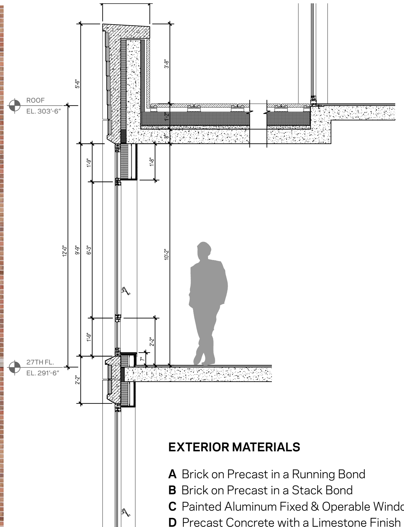
2 SECTION 3/8" = 1'-0"
