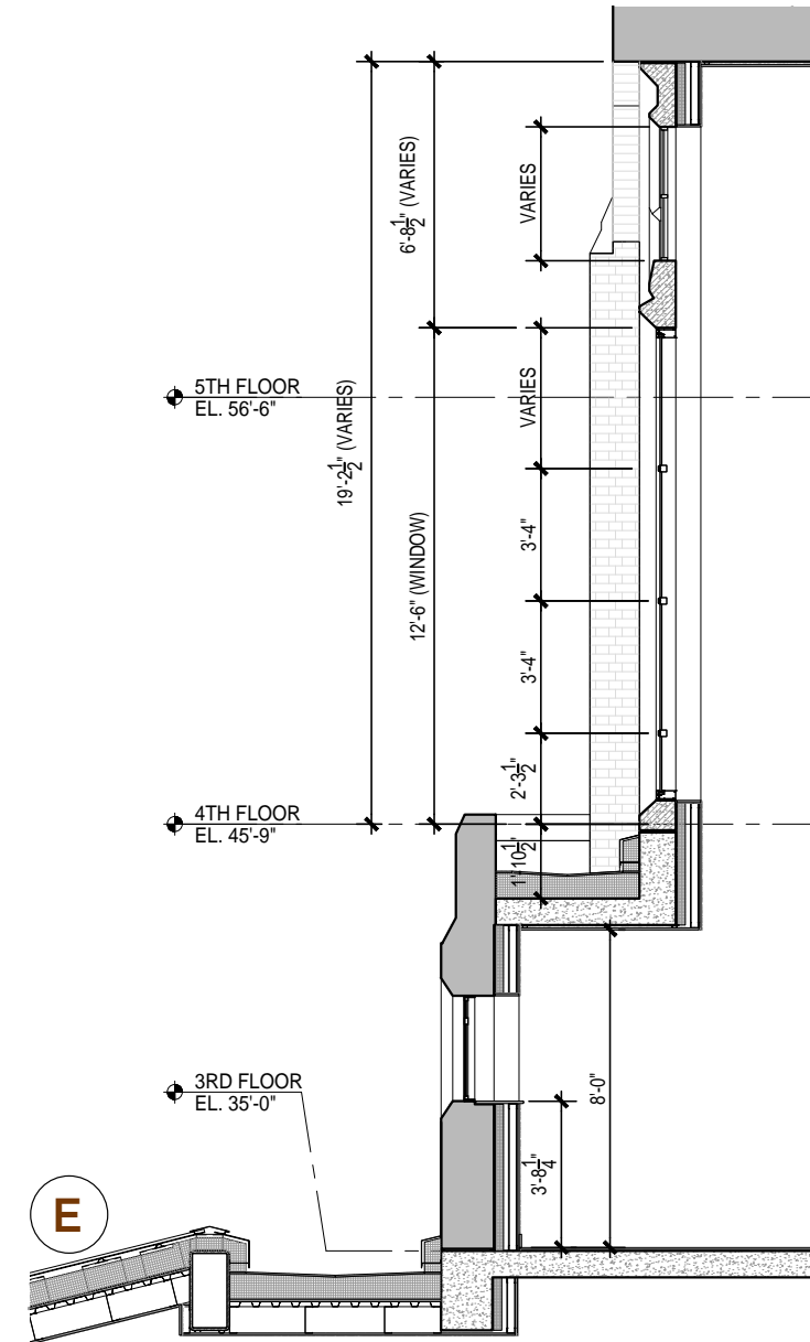
3 SECTION 3/16" = 1'-0"
