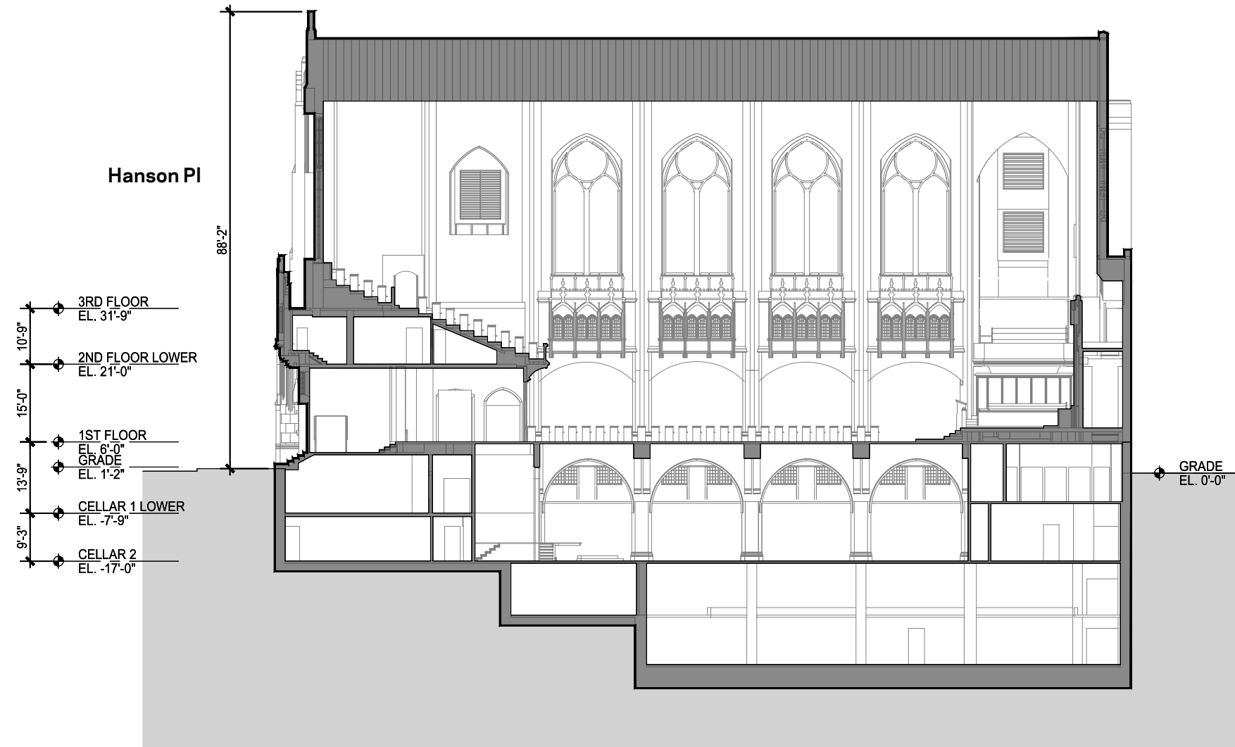
North-South Section
