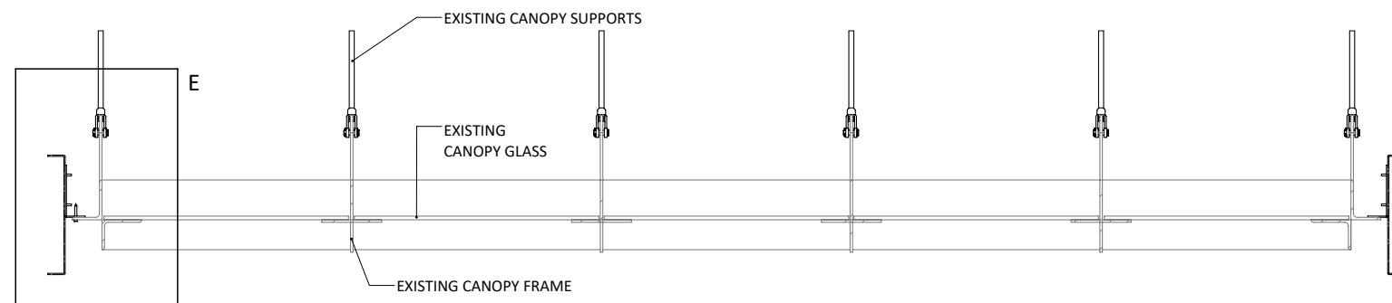
SECTION C-C
