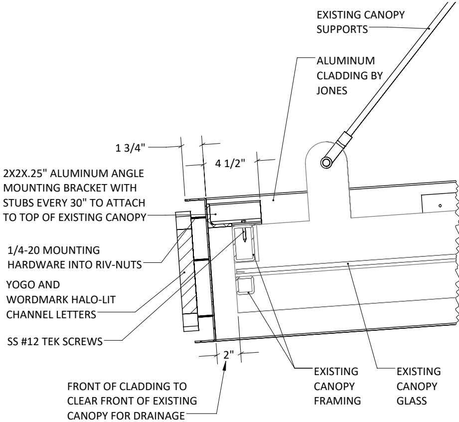
DETAIL D
