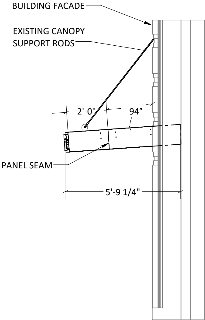
END VIEW
