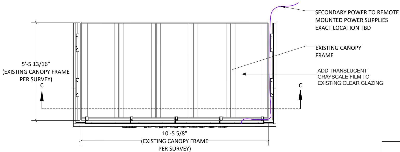
TOP VIEW
