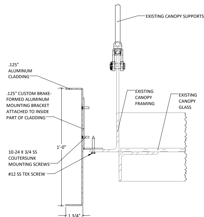
DETAIL E
