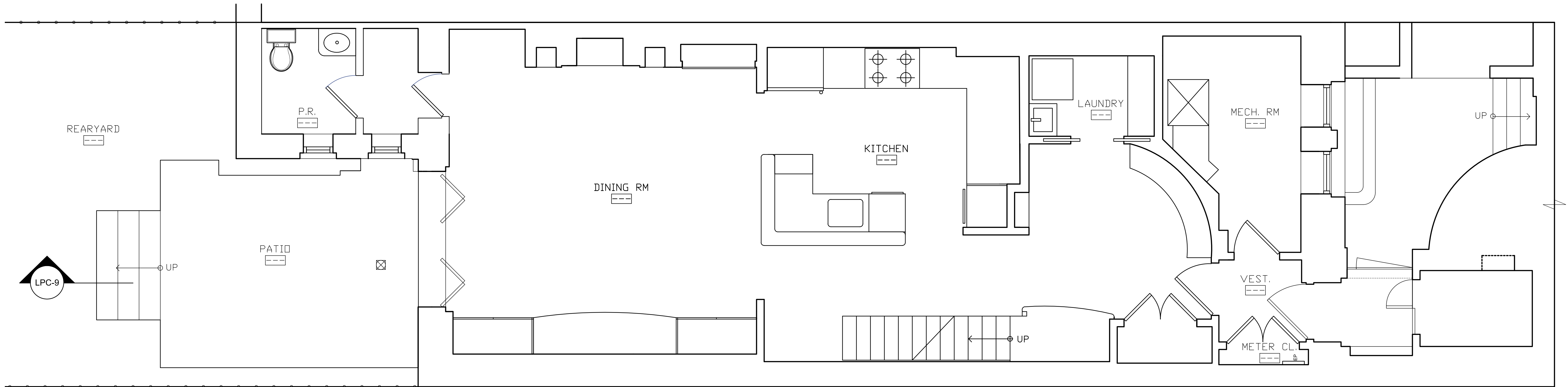
GROUND FLOOR - EXISTING PLAN
