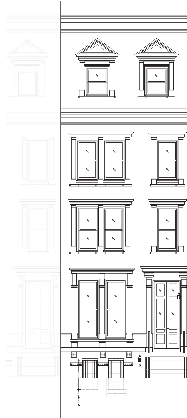
PROPOSED ELEVATION
