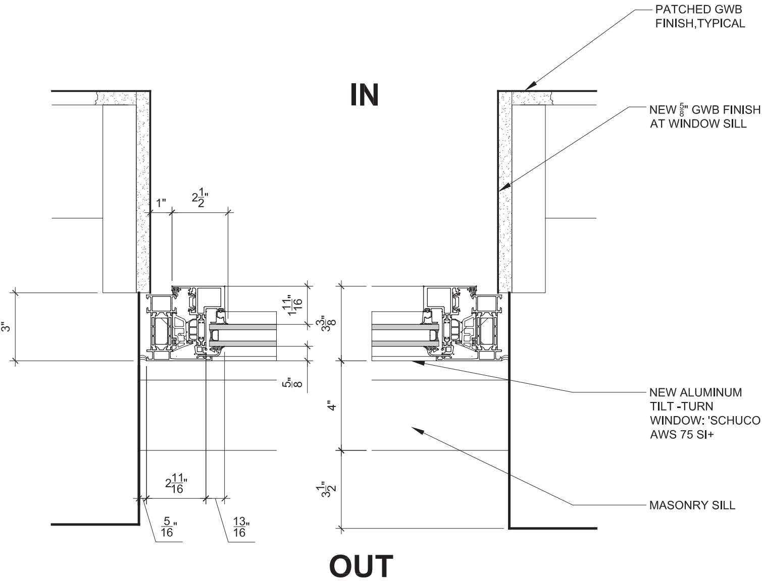
TYPICAL WINDOW PLAN DETAIL
