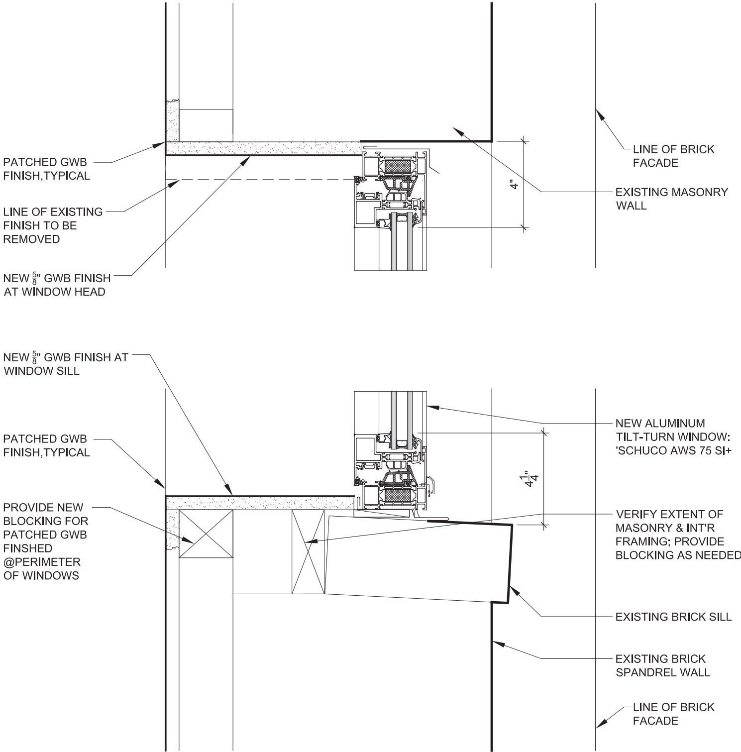
TYPICAL WINDOW SECTION DETAIL
