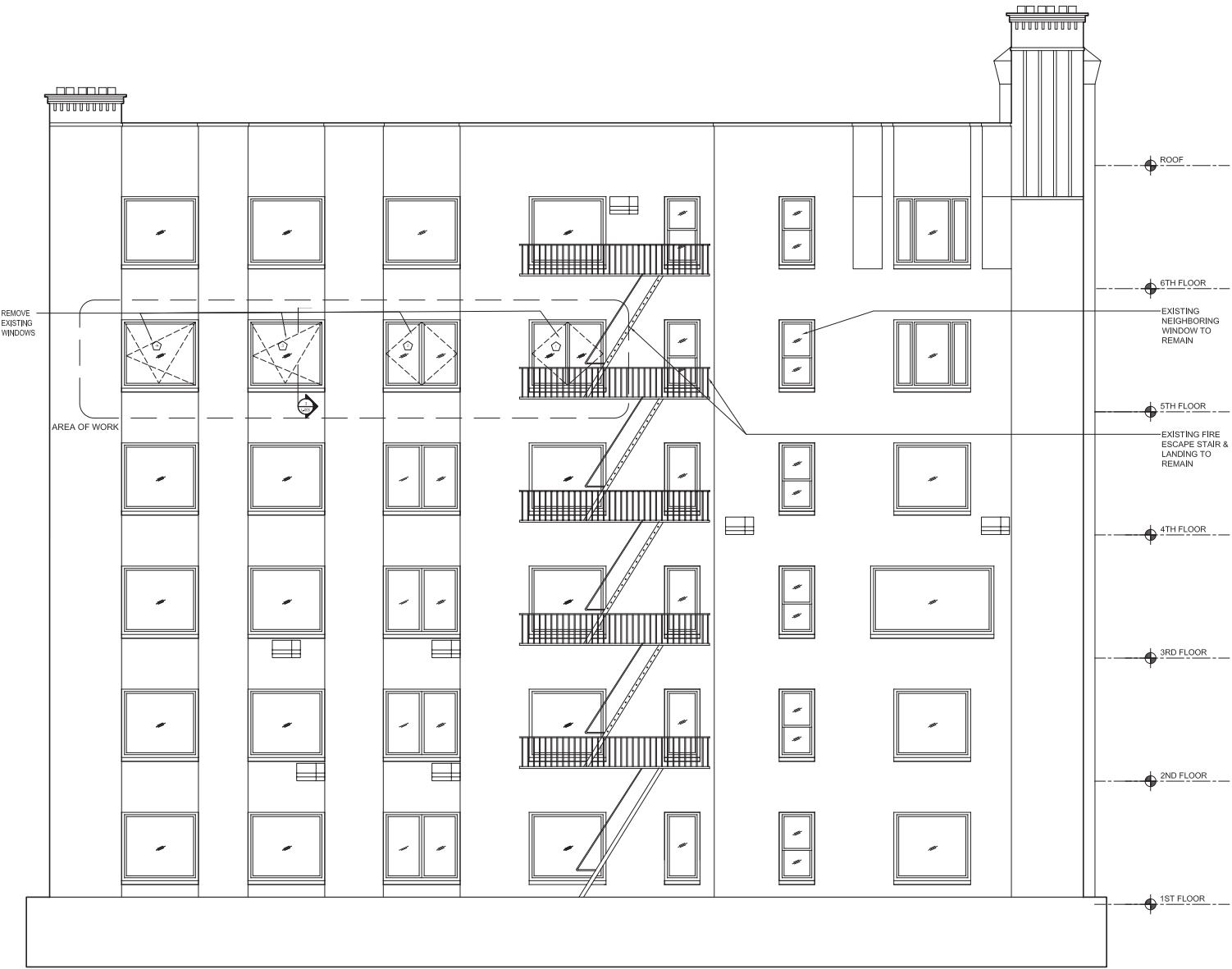
WEST ELEVATION - EXISTING
