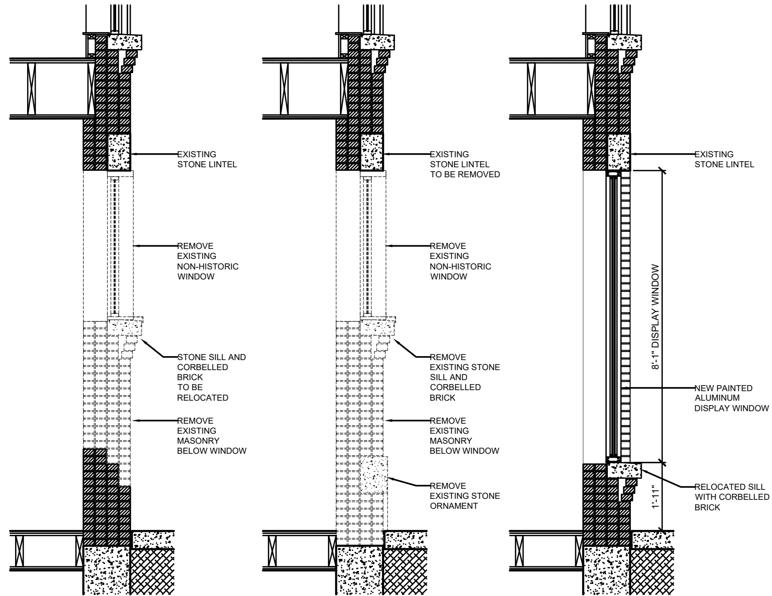
S04 EXISTING SECTION AT GANSEVOORT STREET WINDOW 3/8" = 1'-0"
