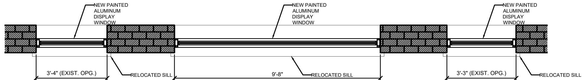
P04 PROPOSED PLAN DETAIL AT GANSEVOORT STREET WINDOW 3/8" = 1'-0"
