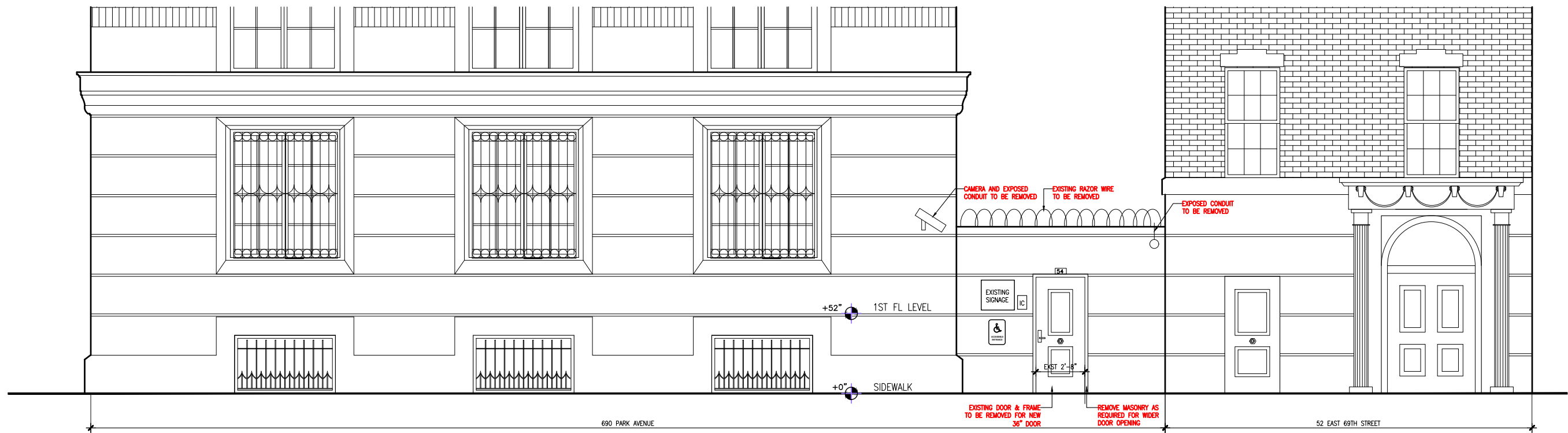
EXISTING STREET ELEVATION
