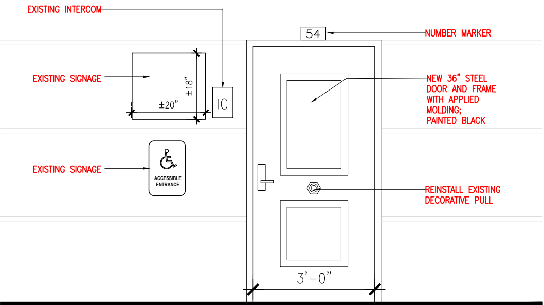
DETAIL OF PROPOSED DOOR
