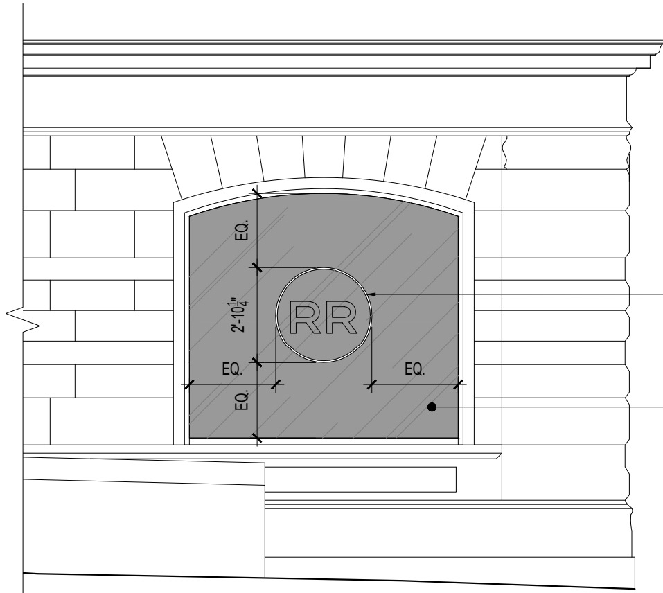
A 69TH ST ELEVATION SCALE: 1/4" = 1'-0"
