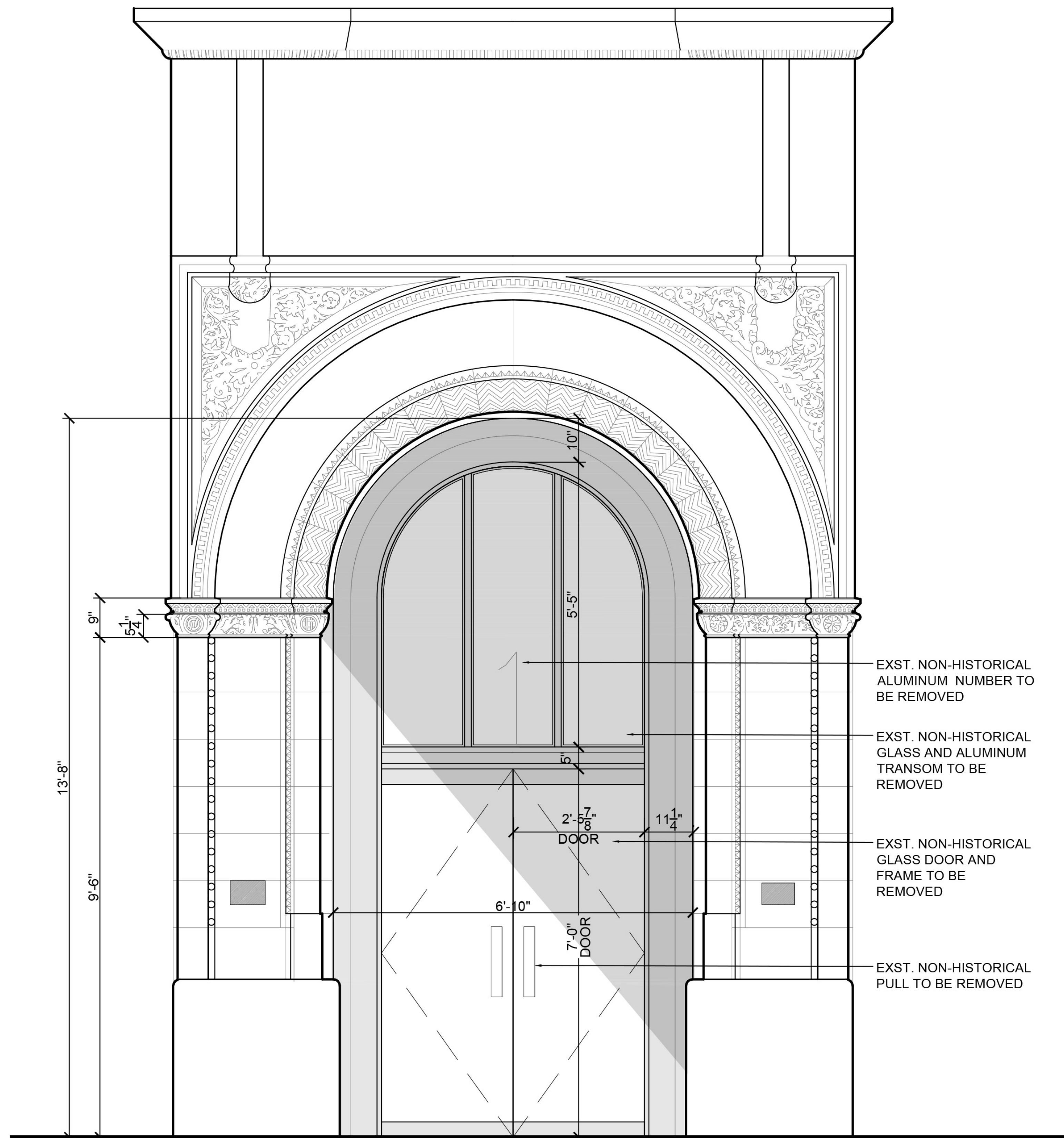
EXISTING ELEVATION
