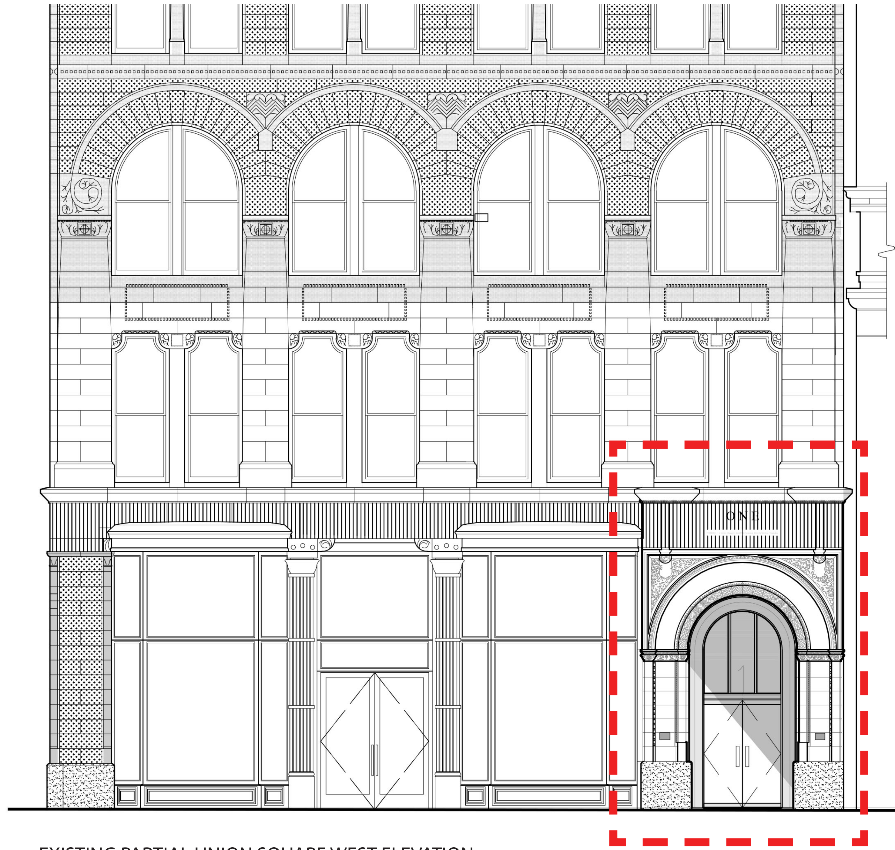
EXISTING PARTIAL UNION SQUARE WEST ELEVATION
