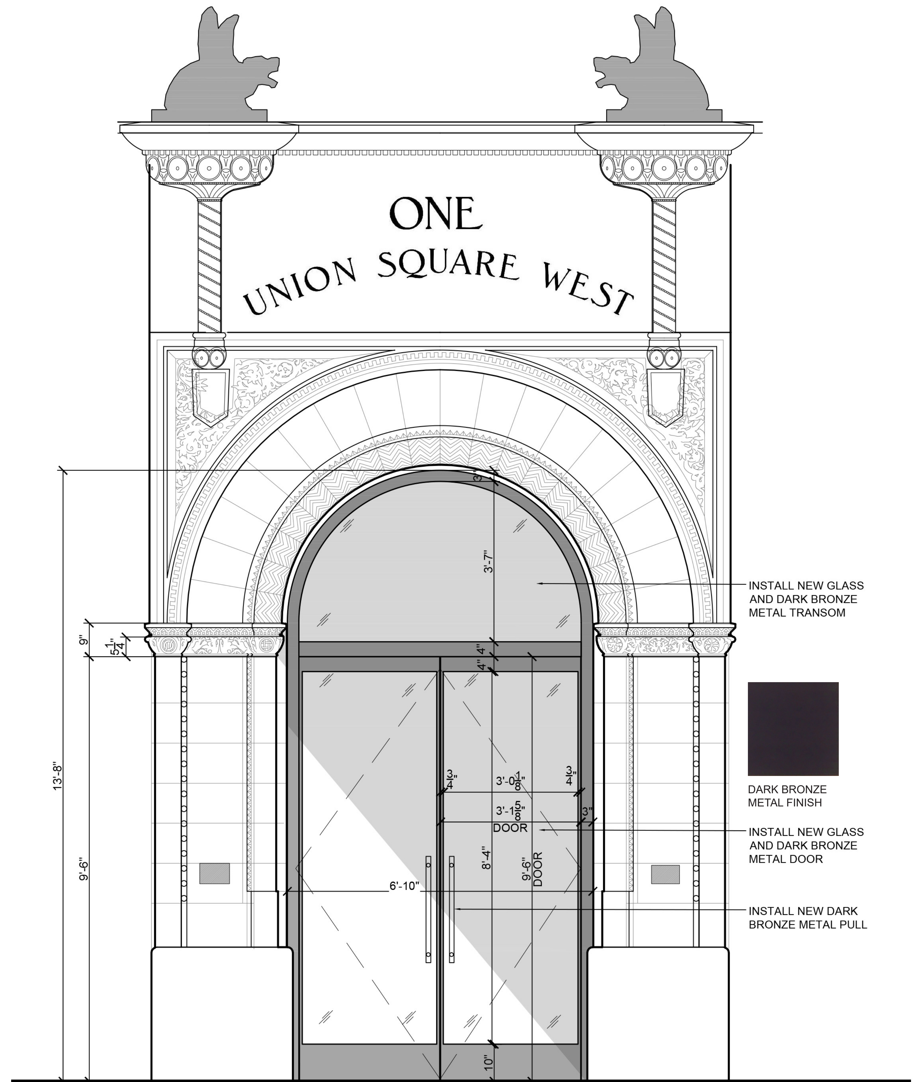
PROPOSED ELEVATION
