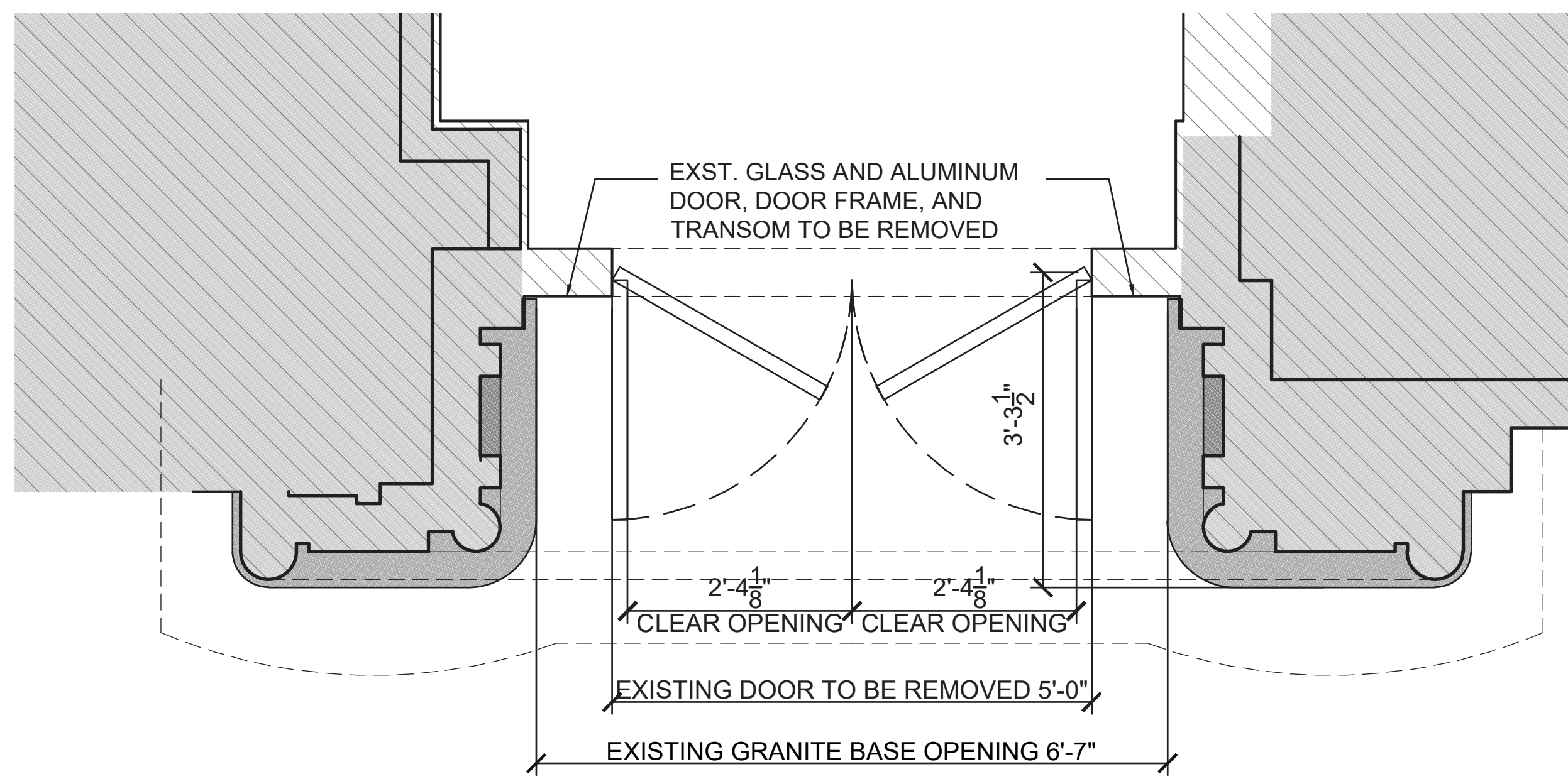
EXISTING PLAN
