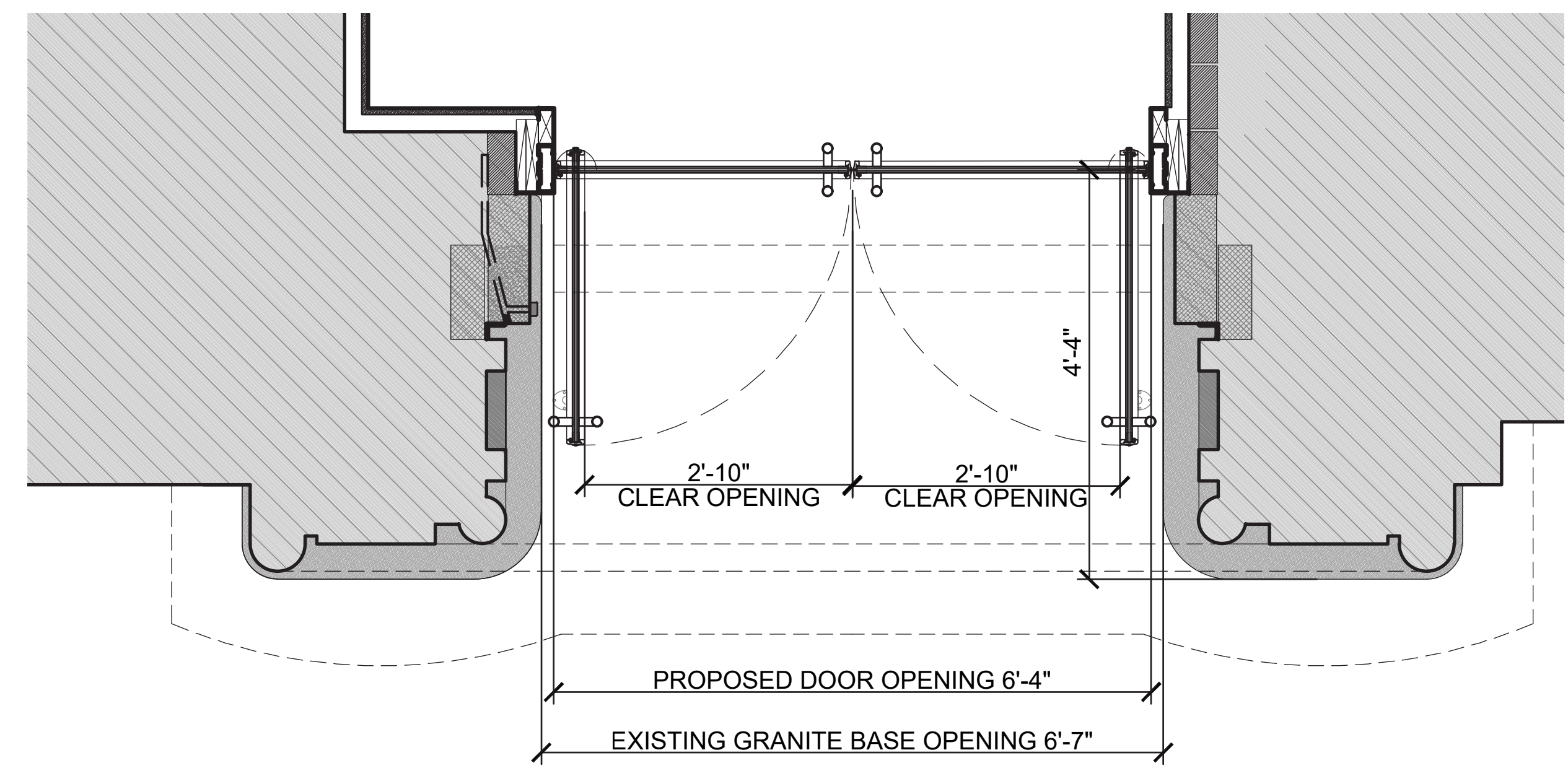
PROPOSED PLAN
