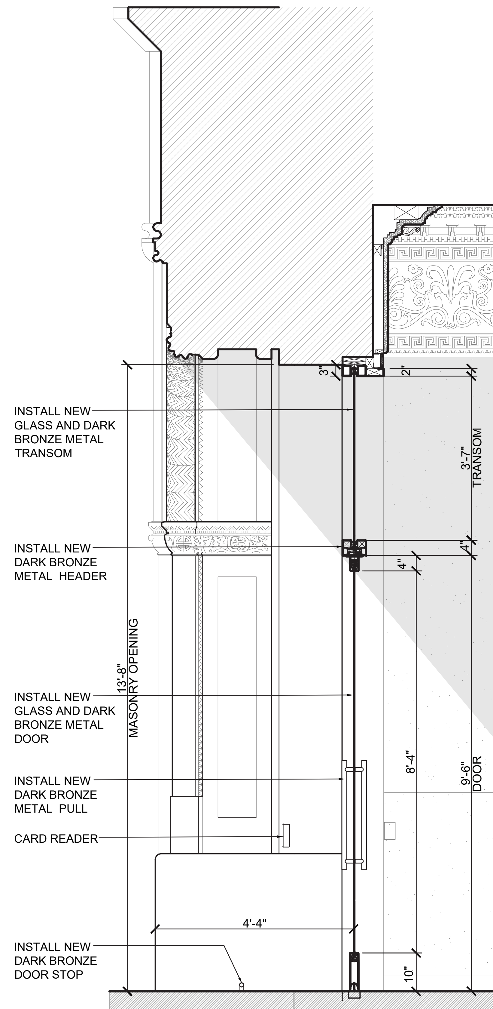
PROPOSED SECTION
