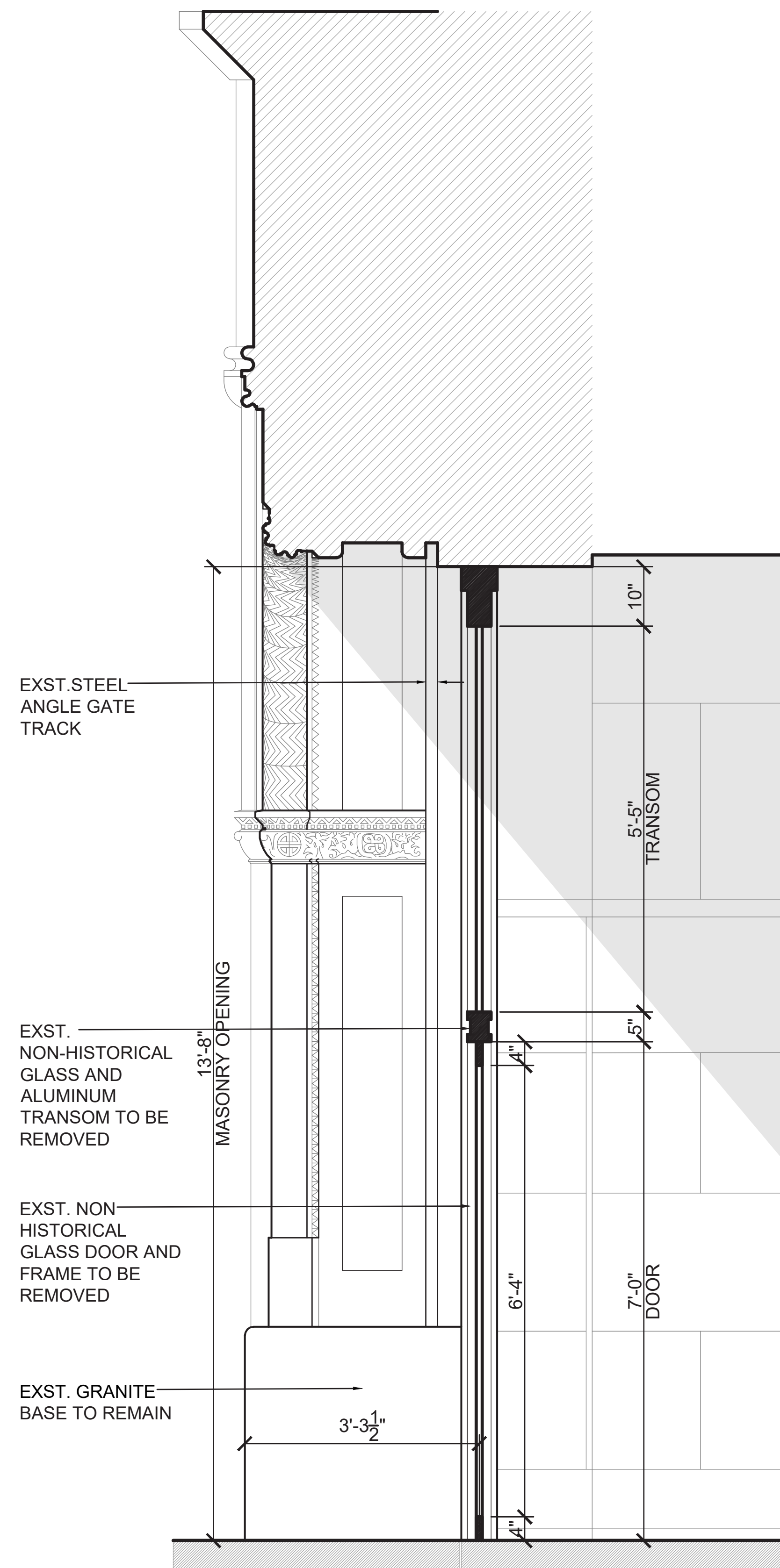
EXISTING SECTION
