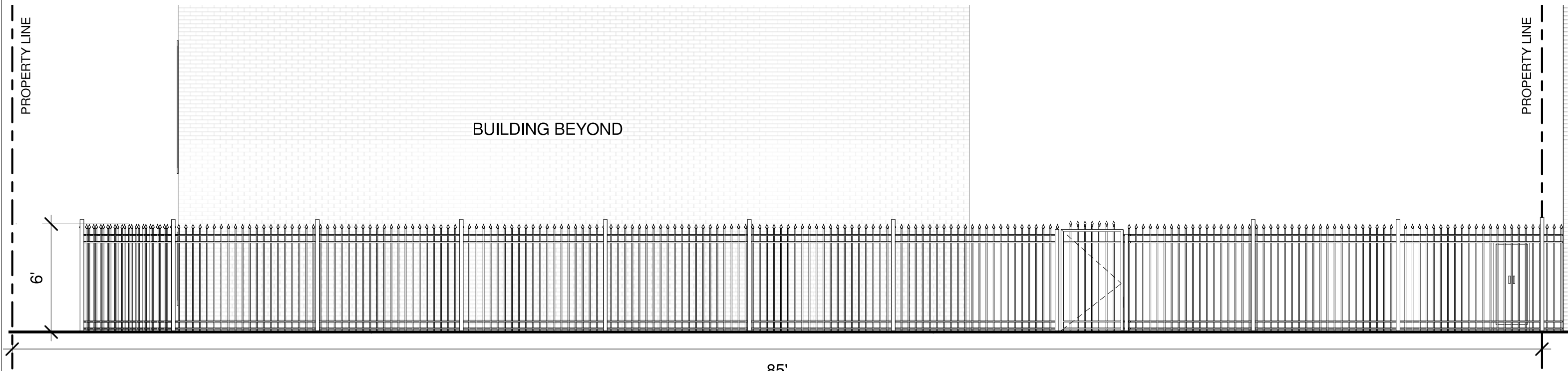
② NORTH ELEVATION 3/16" = 1'-0"
