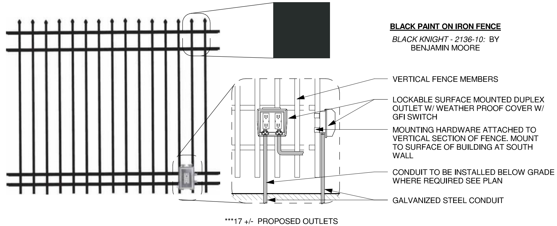
① PROPOSED FENCE 1" = 1'-0"
