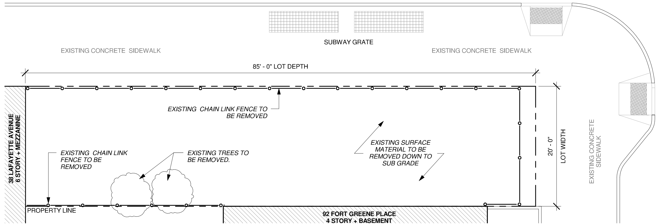
1 EXISTING CONDITIONS 1/8" = 1'-0"
