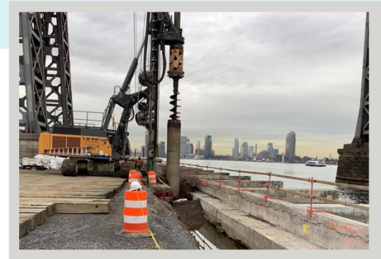
Combi-wall installation underneath Williamsburg Bridge, January 2023
