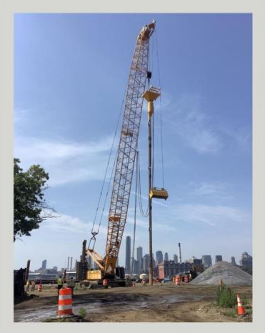
Soil Stabilization at East River Park waterfront, July 2022
