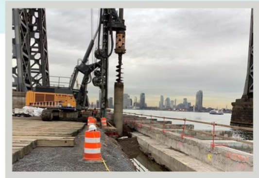
Combi-wall installation underneath Williamsburg Bridge, January 2023
