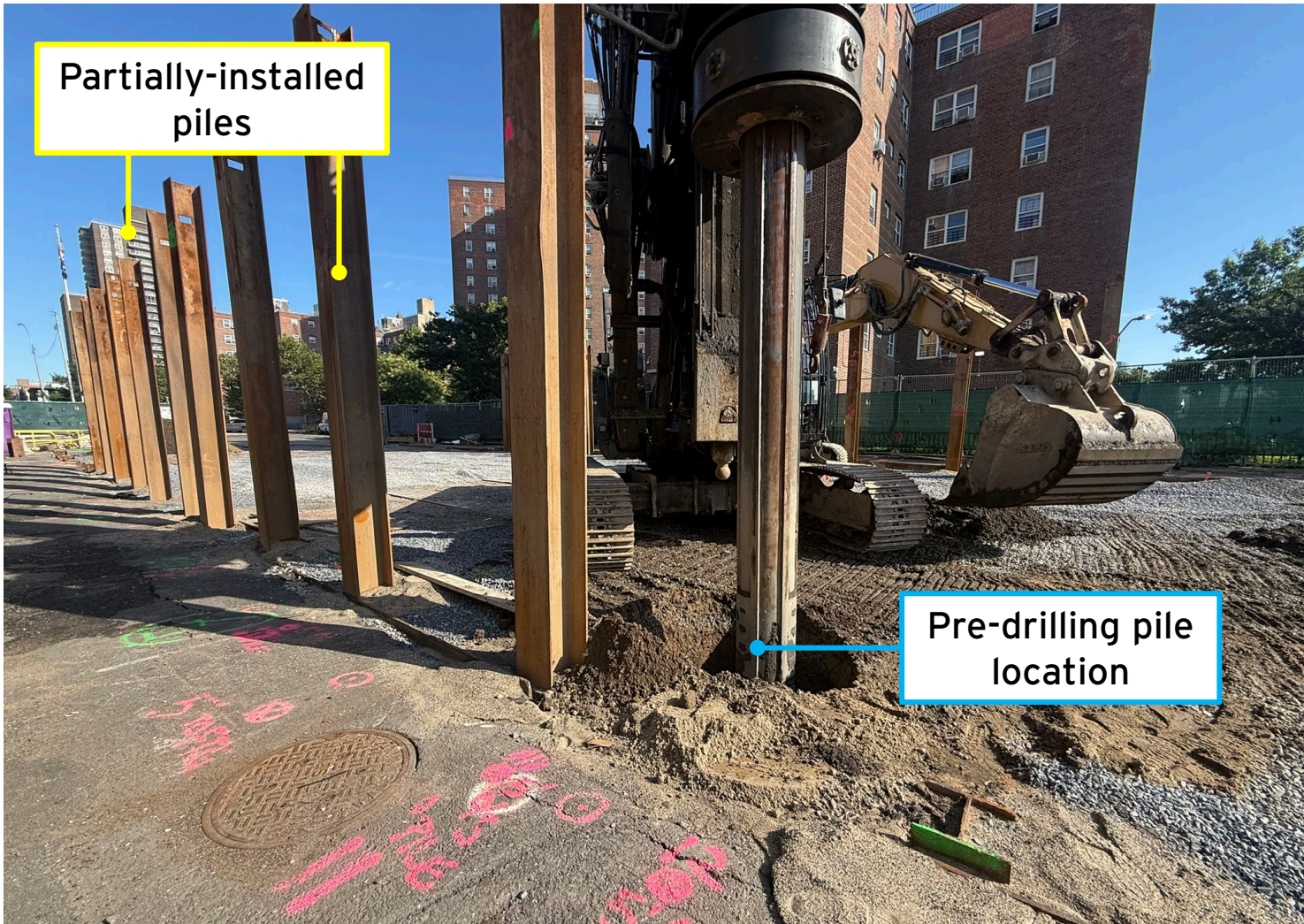
E. 10 th Street bridge pile installation – August 2026
