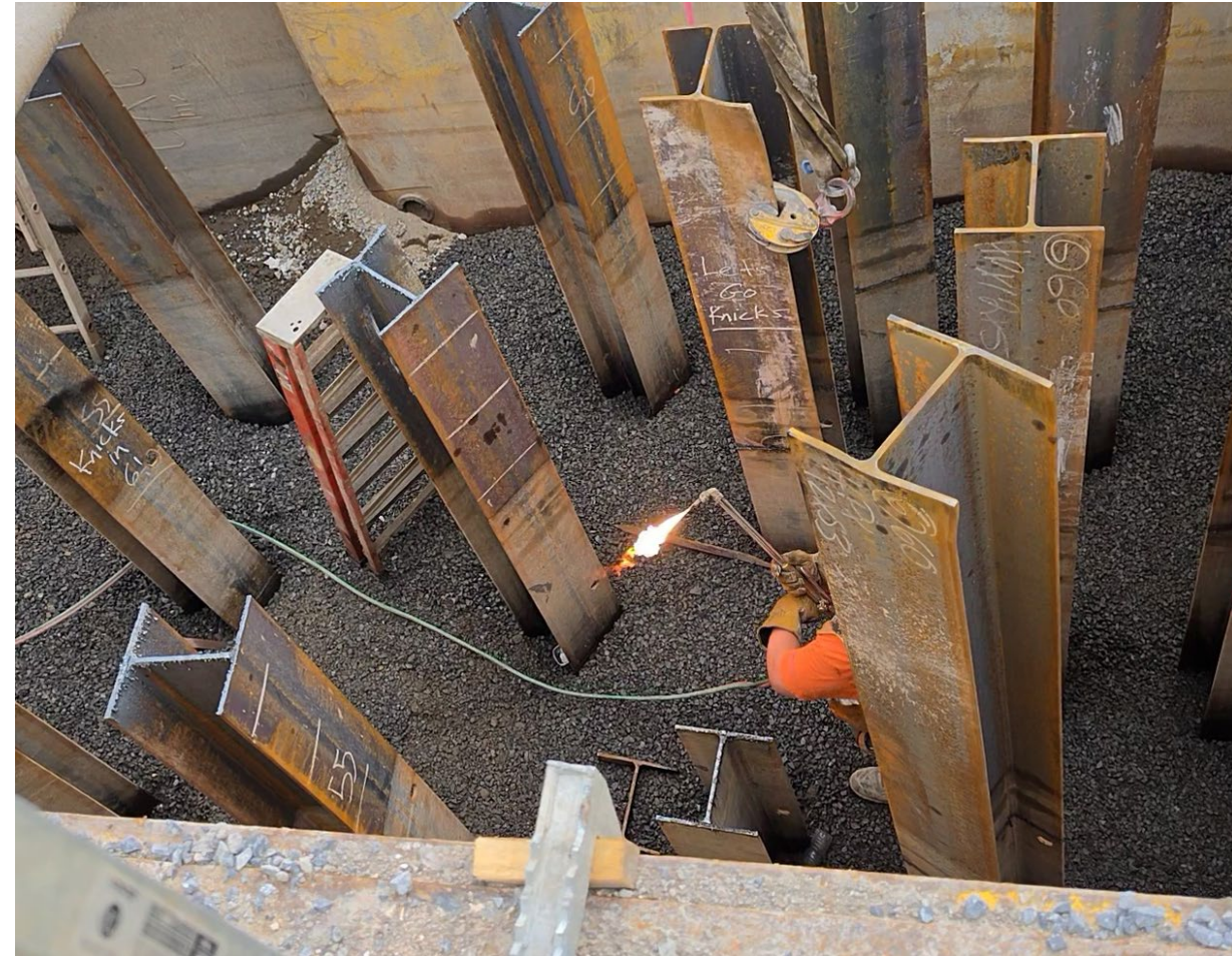
H-piles for sewer support near track area – June 2026
