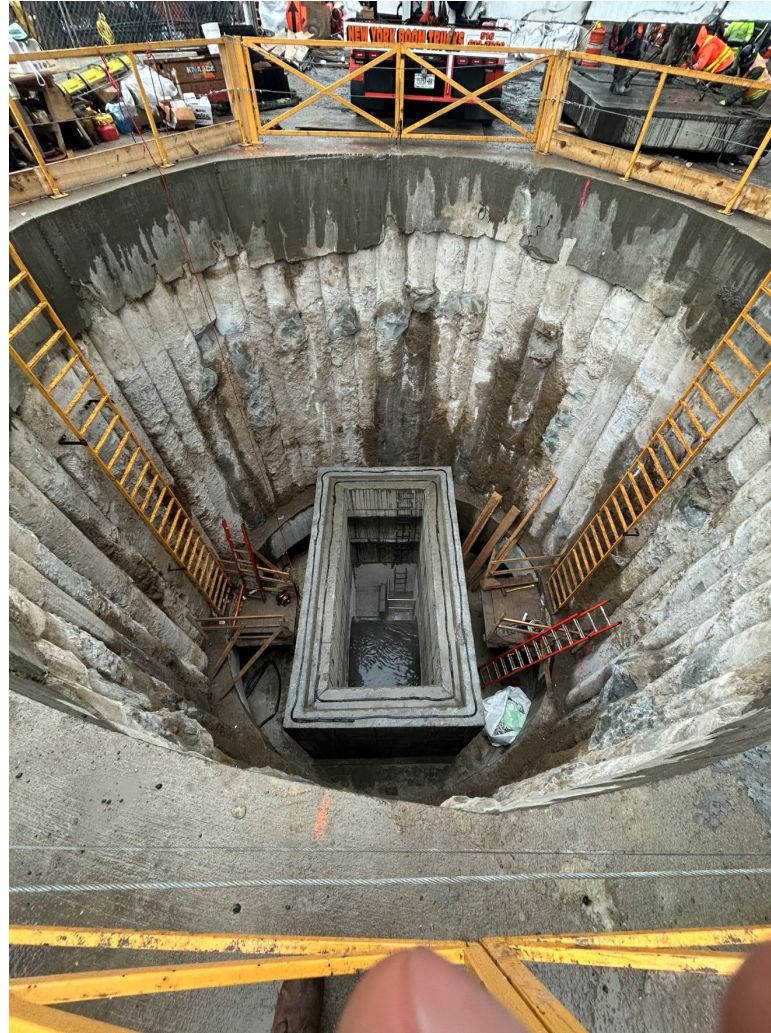
Deep Drop Manhole base installation at Delancey St. S and Baruch Dr. – February 2026
