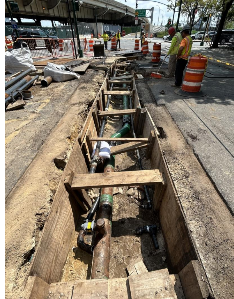
Gas main relocation at E. 18 th Street – September 2025
