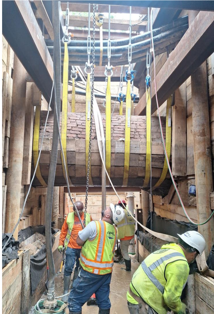
Sewer installation in Jackson Street – September 2025
