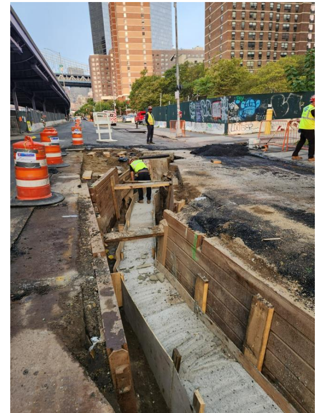
Electrical conduit installation on South Street – September 2025
