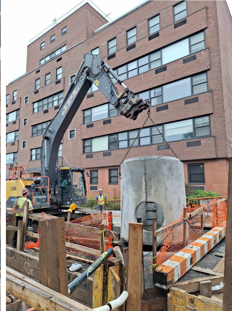
Manhole installation in Jackson Street – September 2025
