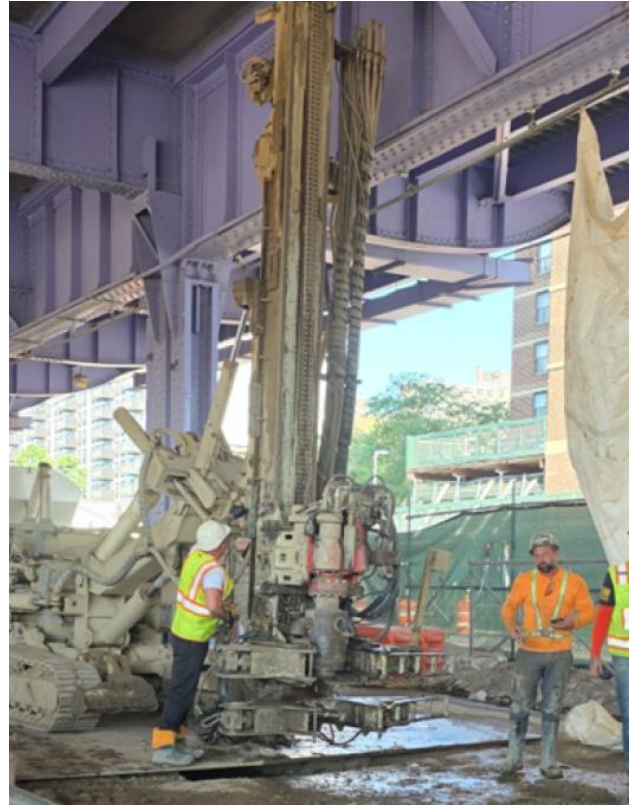
Micropile installation under FDR Drive – September 2025
