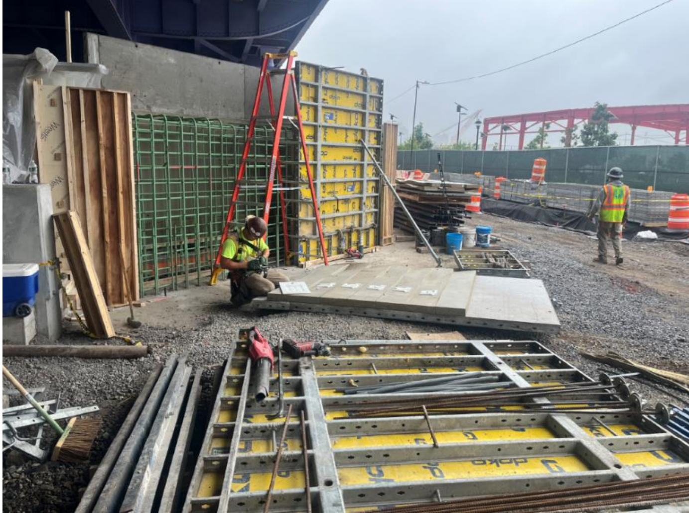
Floodwall formwork adjacent to FDR ramp / Pier 42 – September 2025
