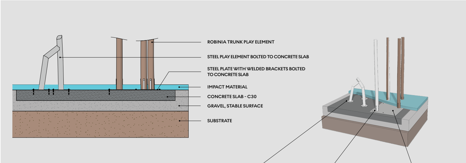
MOUNTING ON A CONCRETE SLAB
