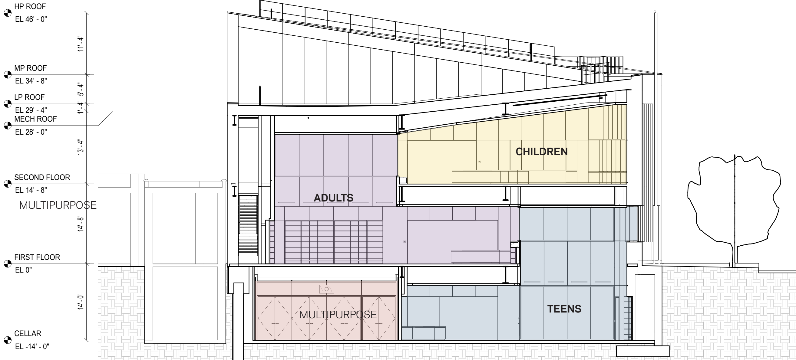
SECTION THROUGH READING ROOMS
