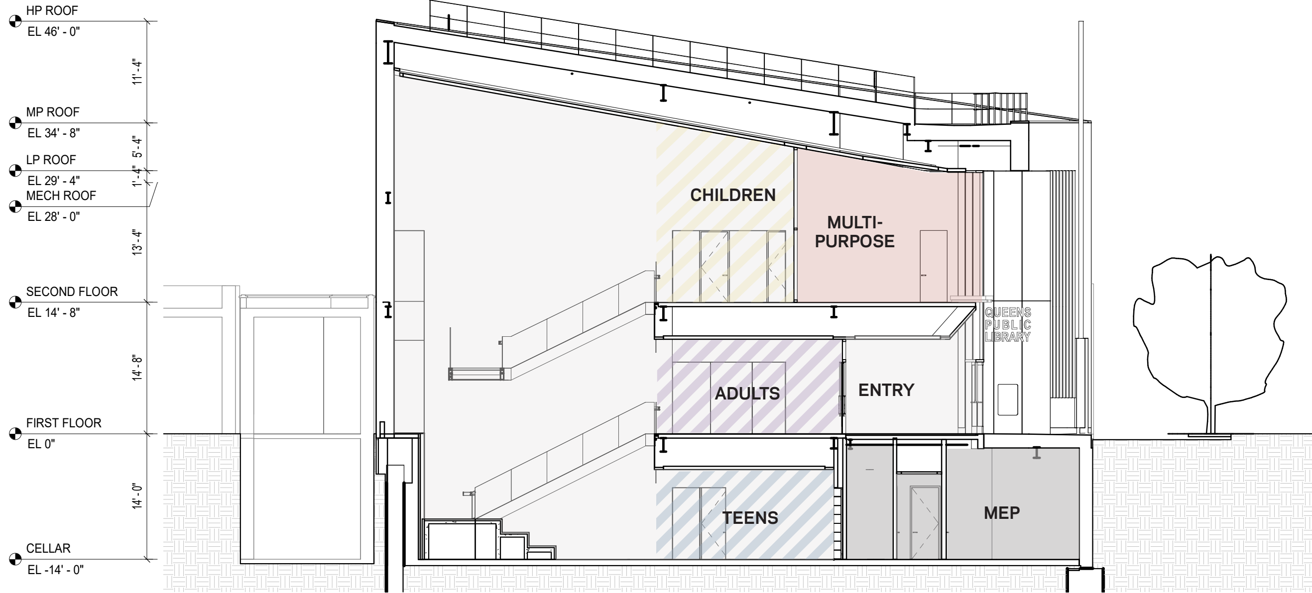
SECTION THROUGH CIRCULATION
