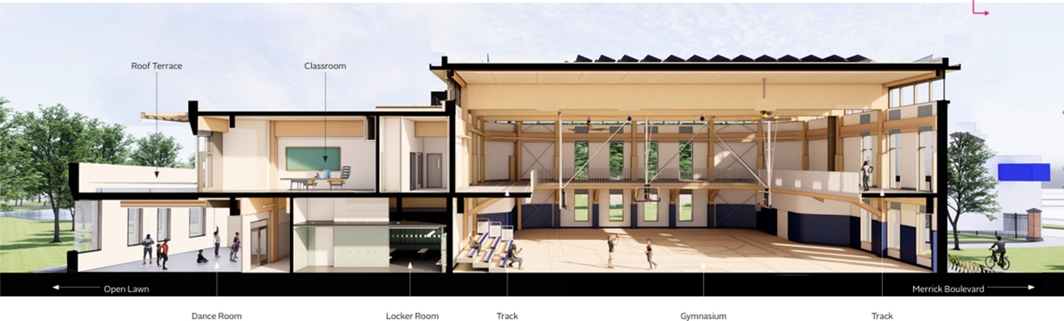
West-East Section
