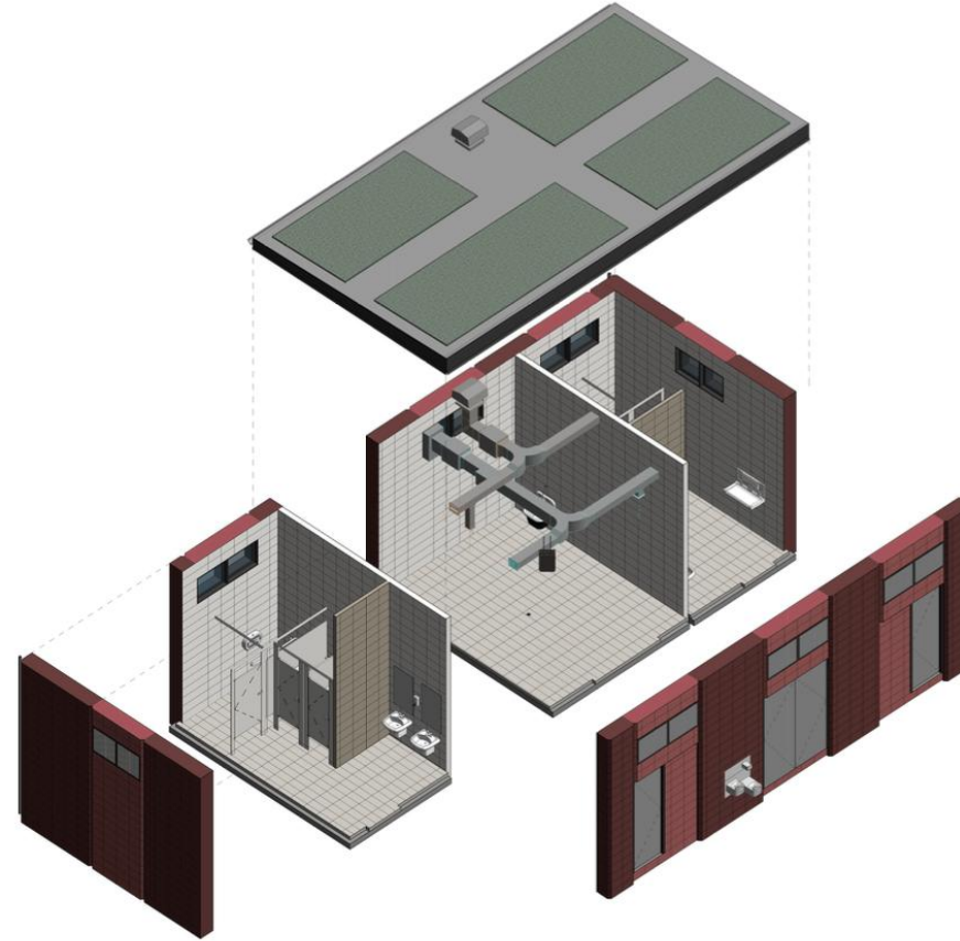
3 EXPLODED AXONOMETRIC EPR-4022.03
