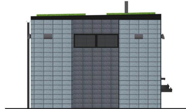
1 - Side Elevation (East)
