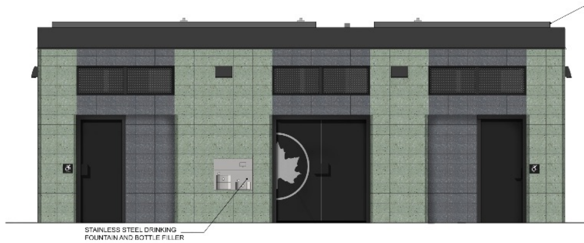
1 - Front Elevation
