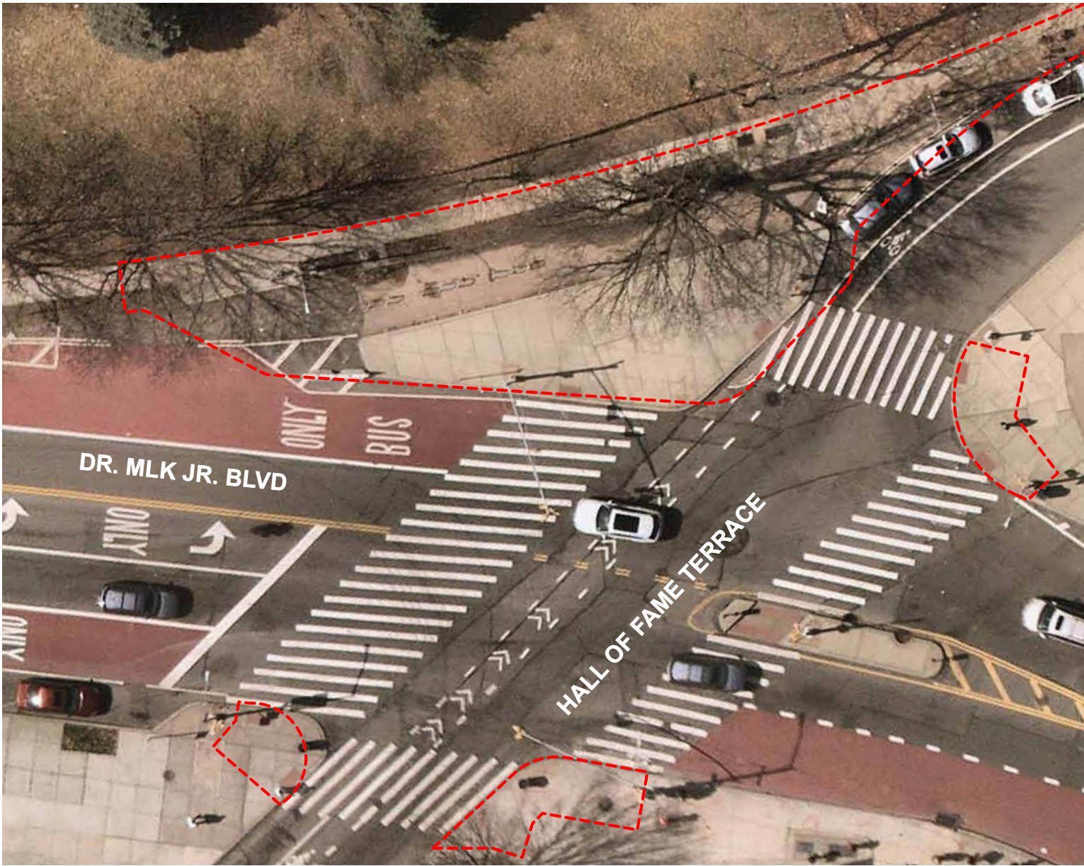
Legend | - - - Schematic Design Curb Line Dr. MLK Jr. Boulevard & Hall of Fame Terrace Existing Conditions 0 20' 40'
