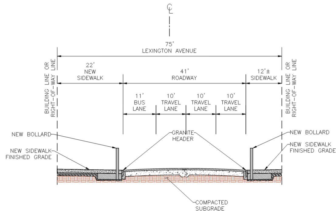
LEXINGTON AVENUE TYPICAL SECTION WITH RAISED INTERSECTION N.T.S.
