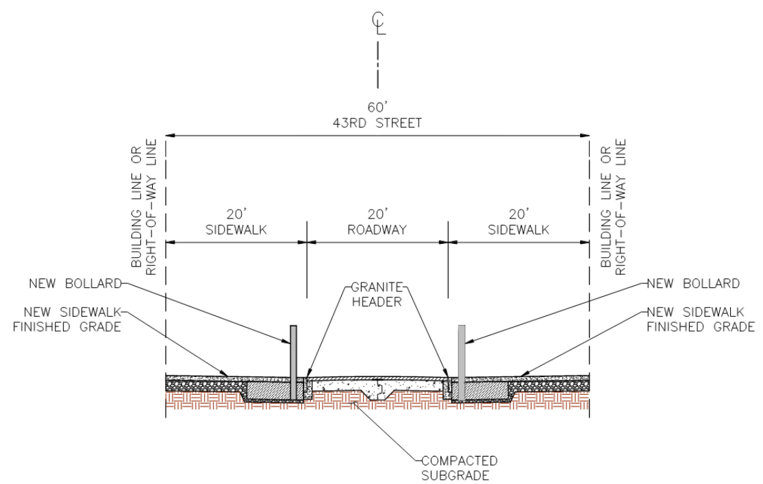
43RD STREET TYPICAL SECTION WITH RAISED INTERSECTION N.T.S.
