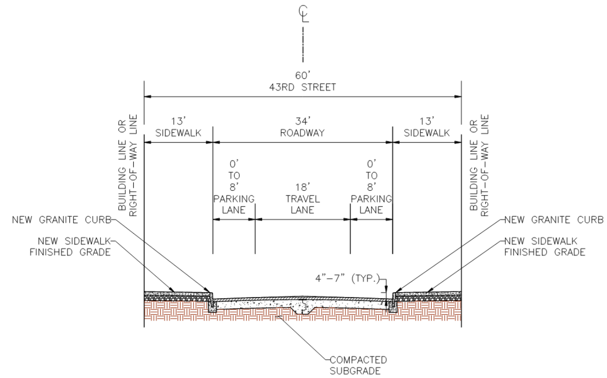
43RD STREET TYPICAL SECTION N.T.S.
