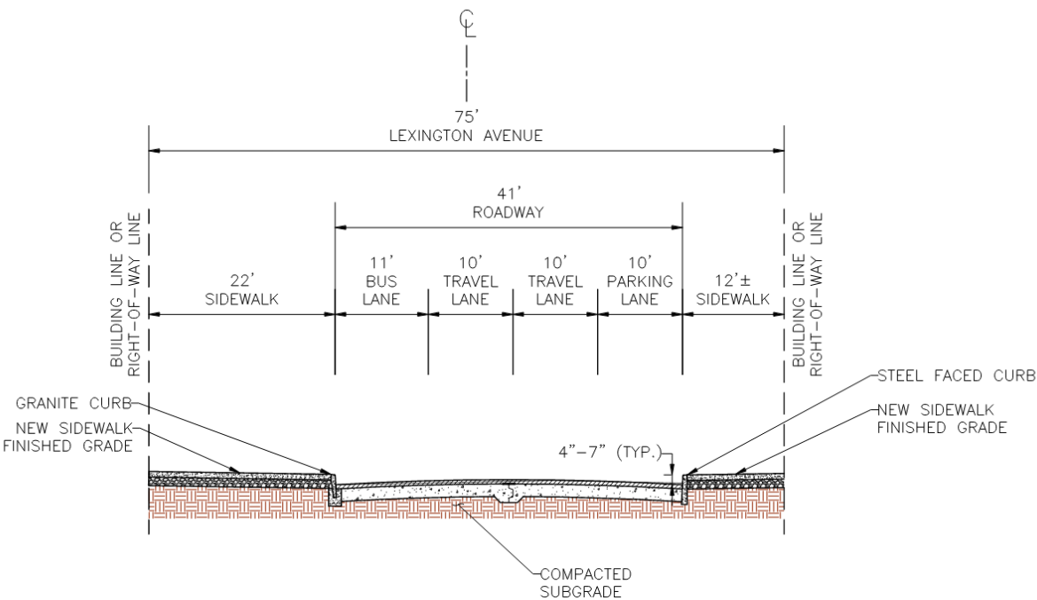
LEXINGTON AVENUE TYPICAL SECTION N.T.S.
